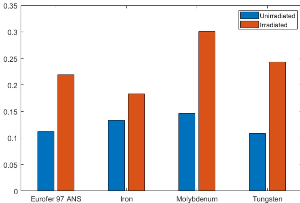
Figure 10 Increase in BDTT in BCC metals following neutron irradiation. Eurofer 97 ANL was irradiated to 16.3 dpa at 573 K [56], molybdenum to 2.2 dpa at 782 K [57] and iron to 0.4 dpa at 678 K [58]
