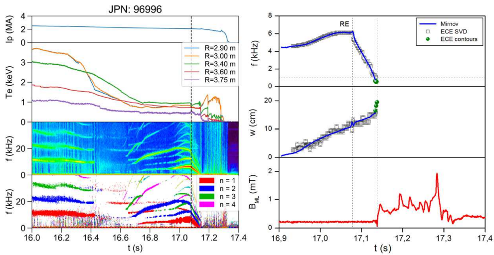
Figure 2. (Left) Time traces of the plasma termination of a pulse with temperature hollowing only. From top to bottom: plasma current, electron temperature at different radii, spectrogram of a magnetic pick-up coil, toroidal mode number analysis from a magnetic pick-up coil array. (Right) Time traces of the n = 1 mode frequency and island width from Mirnov coils and from SVD analysis, and of the n = 1 mode lock amplitude from saddle flux loops for the last 400 ms to disruption. A direct estimation of the island with from ECE contours for the last 5 ms to mode lock has been also added (green symbols). JPN 96996.
