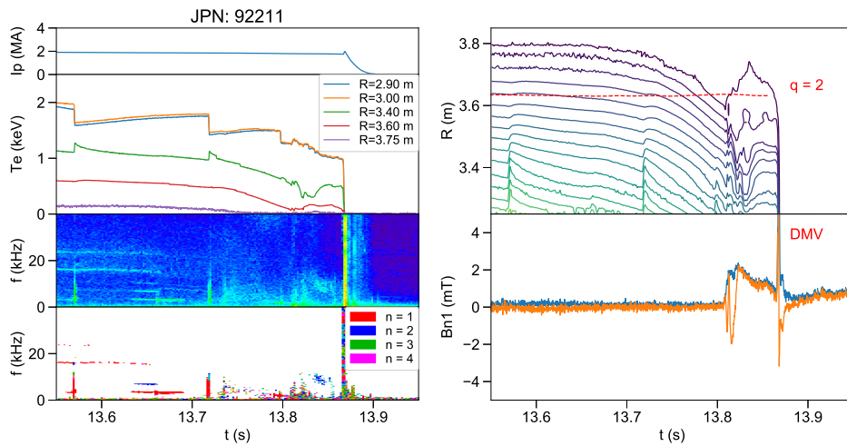
Figure 3. (Left) Time traces of the plasma termination of a pulse with edge cooling only. From top to bottom: plasma current, electron temperature at different radii, spectrogram of a magnetic pick-up coil, toroidal mode number analysis from a magnetic pick-up coil array. (Right) Time traces of the electron temperature contours (top) and of n = 1 mode amplitude and sine components on internal discrete coils (bottom) for the last 300 ms to disruption. JPN 92211.
