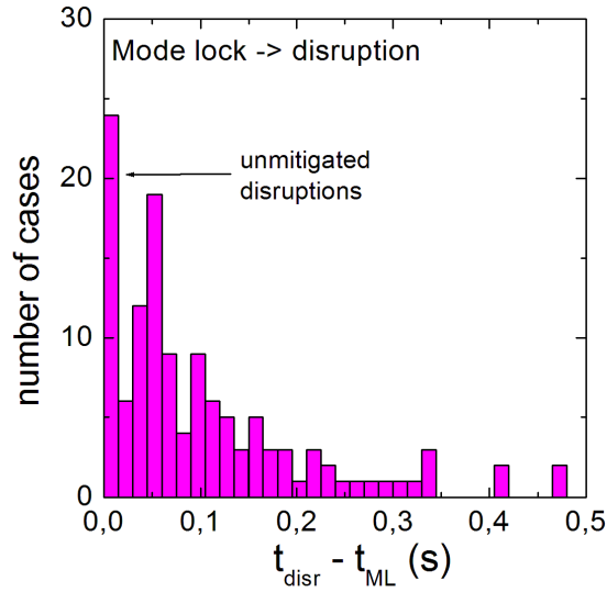
Figure 8. Distribution of the time interval between mode lock ( t_{ML} ) and disruption ( t_{disr} ) for all the disruptive pulses. The first bin (0–15 ms) correspond to unmitigated pulses (thermal quenches before disruption mitigation valve intervention). Longer delays correspond to low amplitude lock modes (triggering late the mitigation actions) and to pulses with sequences of soft disruptions.
