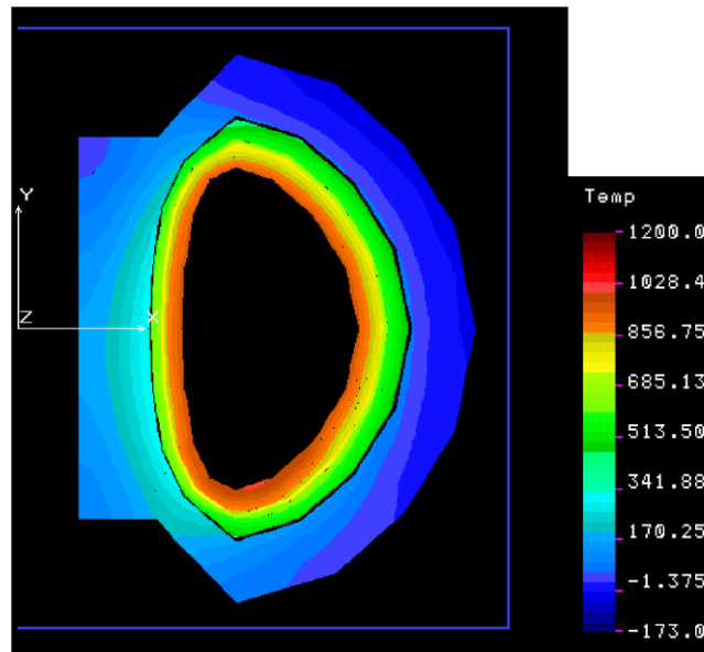
Figure 3: PPCS Model A poloidal temperature profile 10 days after a total LOCA occurs [6]. Note, the temperature scale is in degrees Celsius and Y denotes the vertical direction
