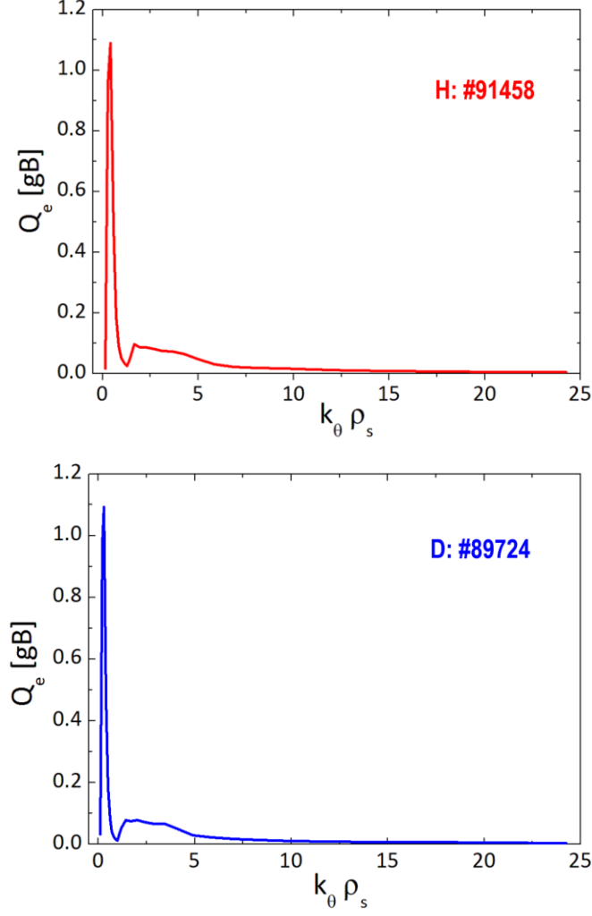
Figure 7. Electron heat flux spectra (in gyro-Bohm units, normalized to D mass) from TGLF at \rho_{tor} = 0.56 , for H (#91458) and D (#89724) L-mode shots, corroborating the finding that ITGs are the dominant instabilities in the plasma core, for both isotopes.
