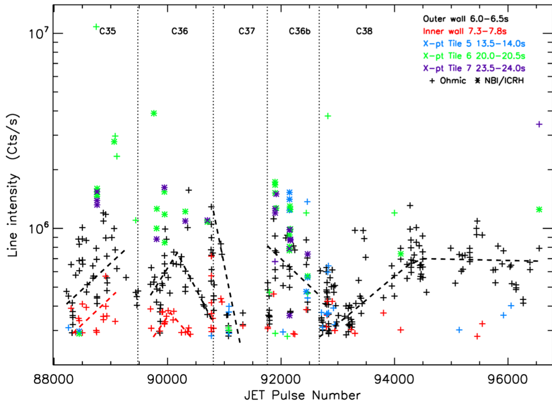
Figure 19. W intensity indicator observed by KT2.
