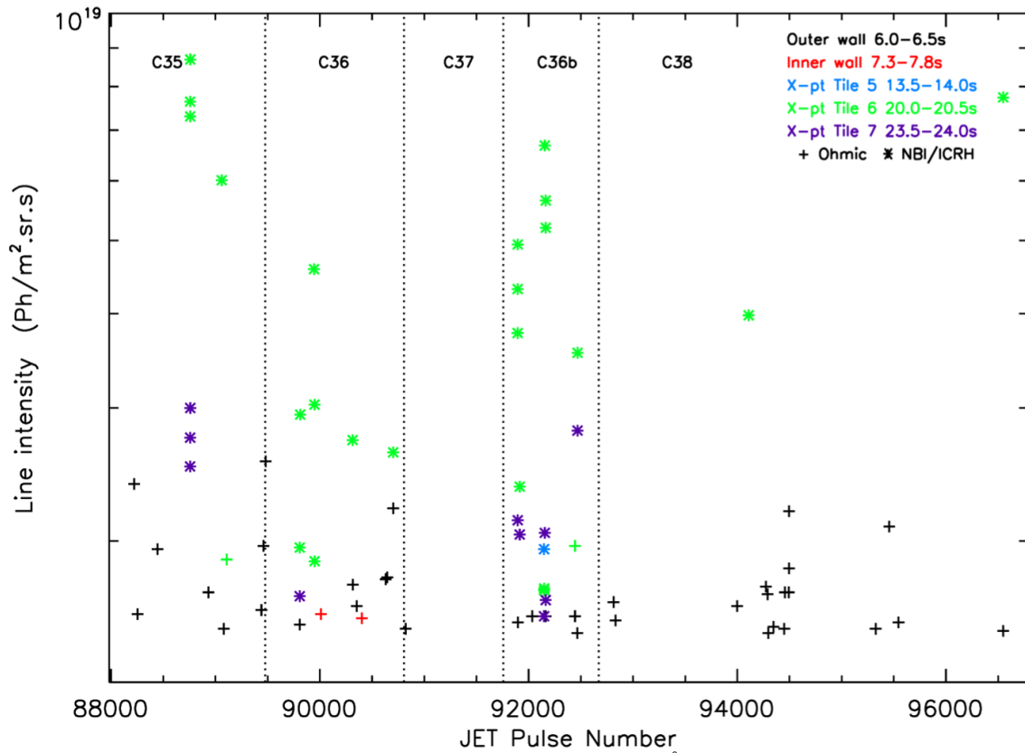
Figure 18. Mo XXXII line intensities at 127.87 Å observed by KT2.
