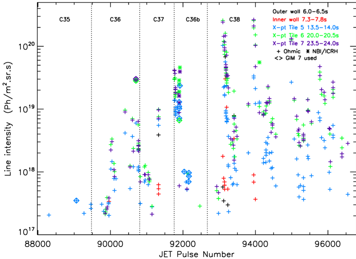
Figure 6. Lyman- \alpha line intensities of He at 303.78 \text{ \AA} observed by KT7/2.
