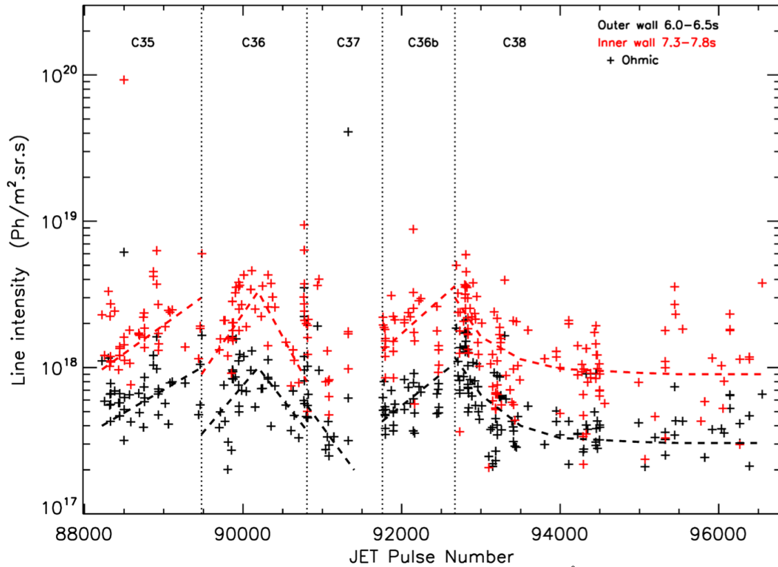
Figure 8a. Outer and inner wall C III line intensities at 977.02 \text{ \AA} observed by KT2.
