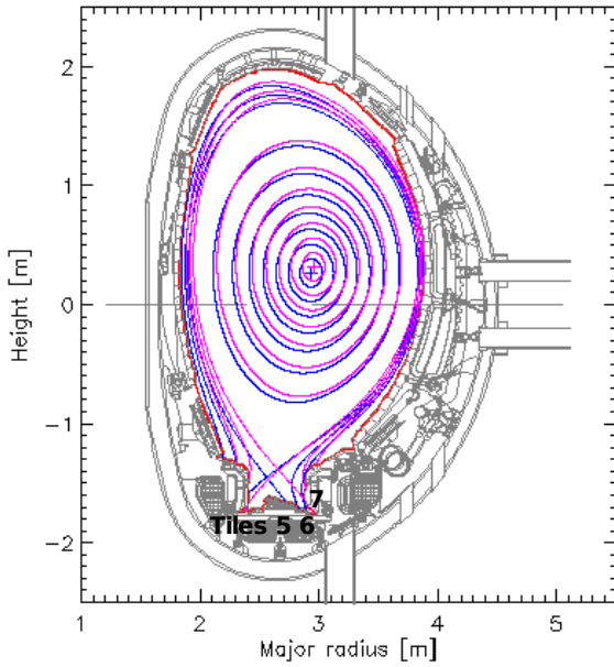
Figure 3. Magnetic configuration of the DiMple pulse 91779 X-point phases with the outer strike point on tile 5 (13.75 s) and tile 7 (23.77 s).
