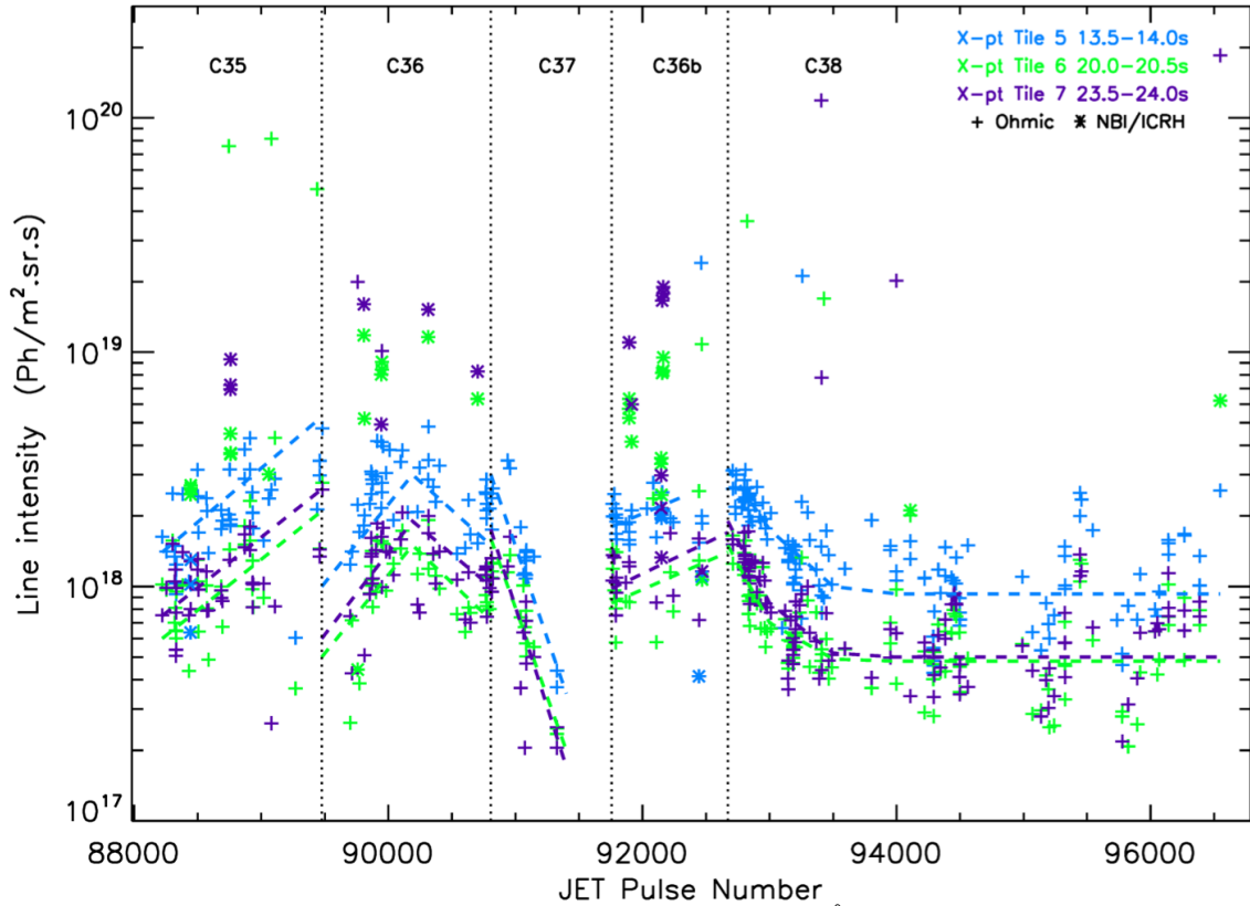
Figure 8b. X-point C III line intensities at 977.02 \text{ \AA} observed by KT2.
