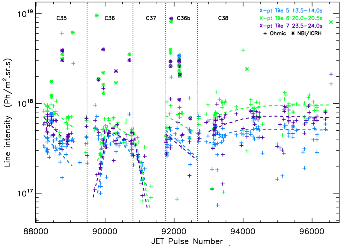
Figure 16b. X-point Fe XVI line intensities at 335.41 \text{ \AA} observed by KT7/2.
