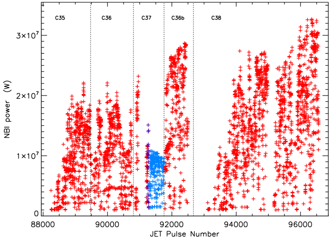
Figure 21. Maximum NBI powers. D beams both octants, octant 4 H octant 8 D , H beams both octants.
