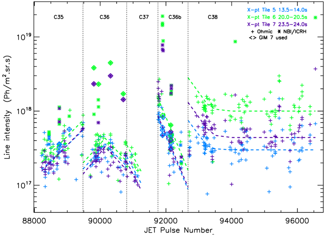
Figure 9b. X-point C IV line intensities at 312.43 Å observed by KT7/2.
