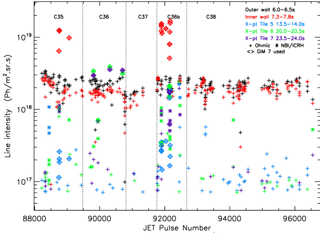
Figure 7. Balmer- \alpha line intensities of Be at 410.06 \text{ \AA} observed by KT7/2.
