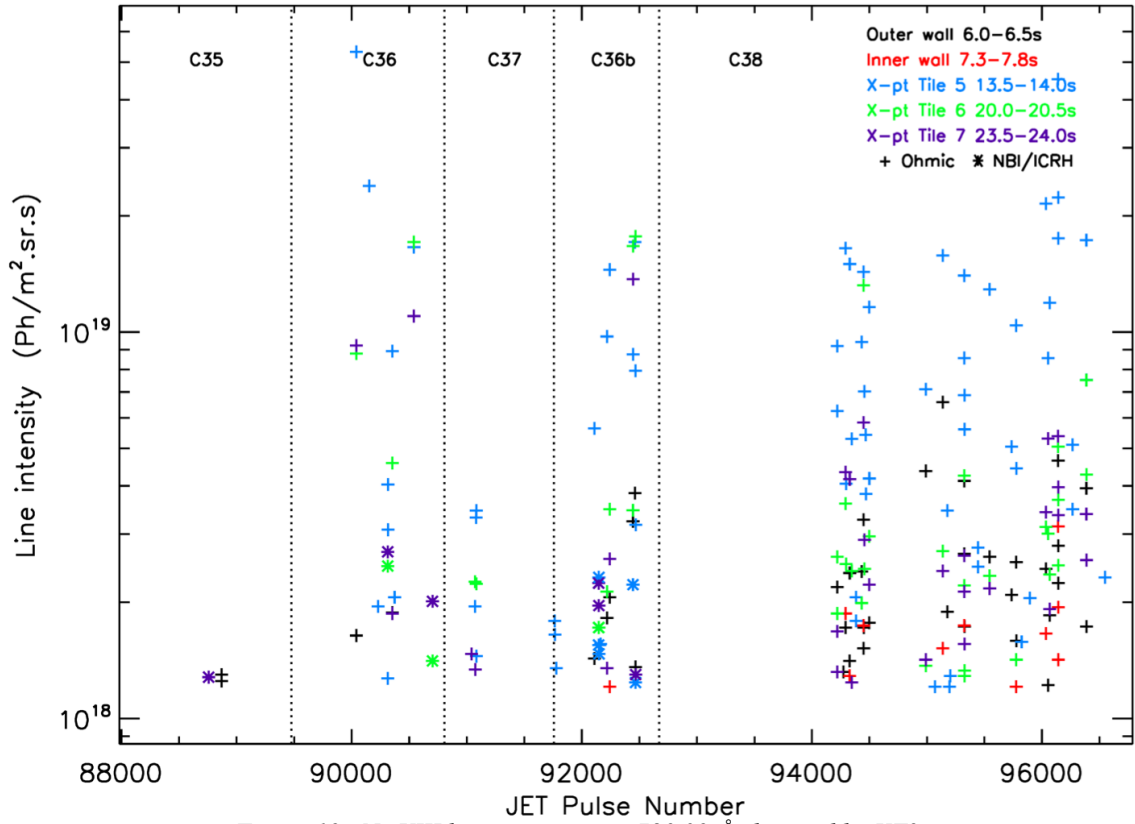
Figure 12. Ne VIII line intensities at 780.32 Å observed by KT2.
