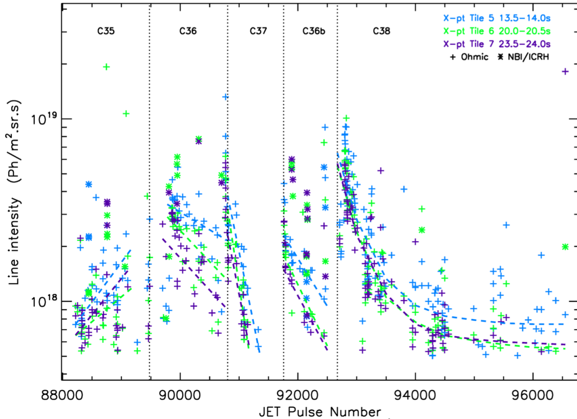
Figure 11b. X-point O V line intensities at 629.73 \text{ \AA} observed by KT2.
