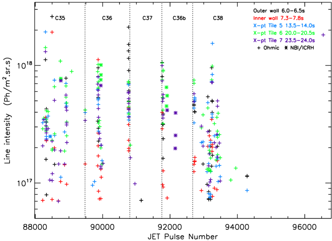
Figure 14. Cl XV line intensities at 415.50 Å observed by KT7/2.
