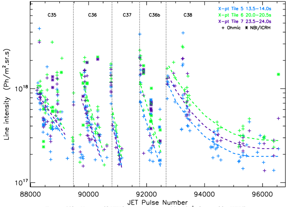
Figure 13b. X-point Cl XIV line intensities at 237.70 Å observed by KT7/2.
