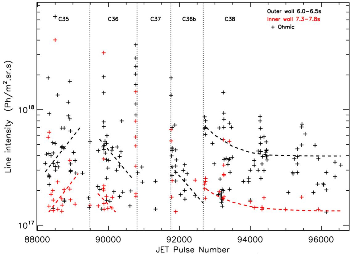
Figure 13a. Outer and inner wall Cl XIV line intensities at 237.70 Å observed by KT7/2.
