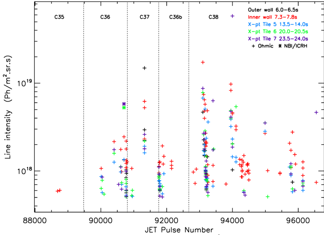
Figure 5. Lyman- \alpha line intensities of He at 303.78 \text{ \AA} observed by KT2.
