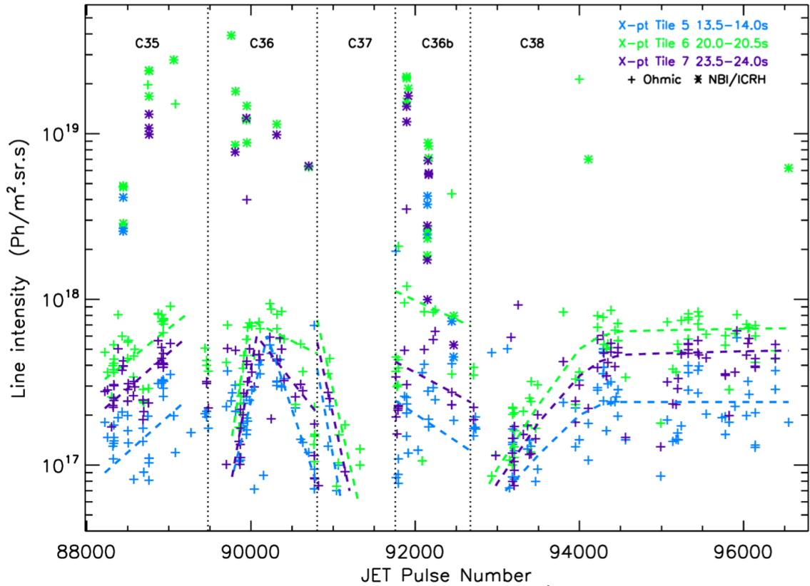
Figure 17b. X-point Cu XIX line intensities at 273.35 \text{ \AA} observed by KT7/2.
