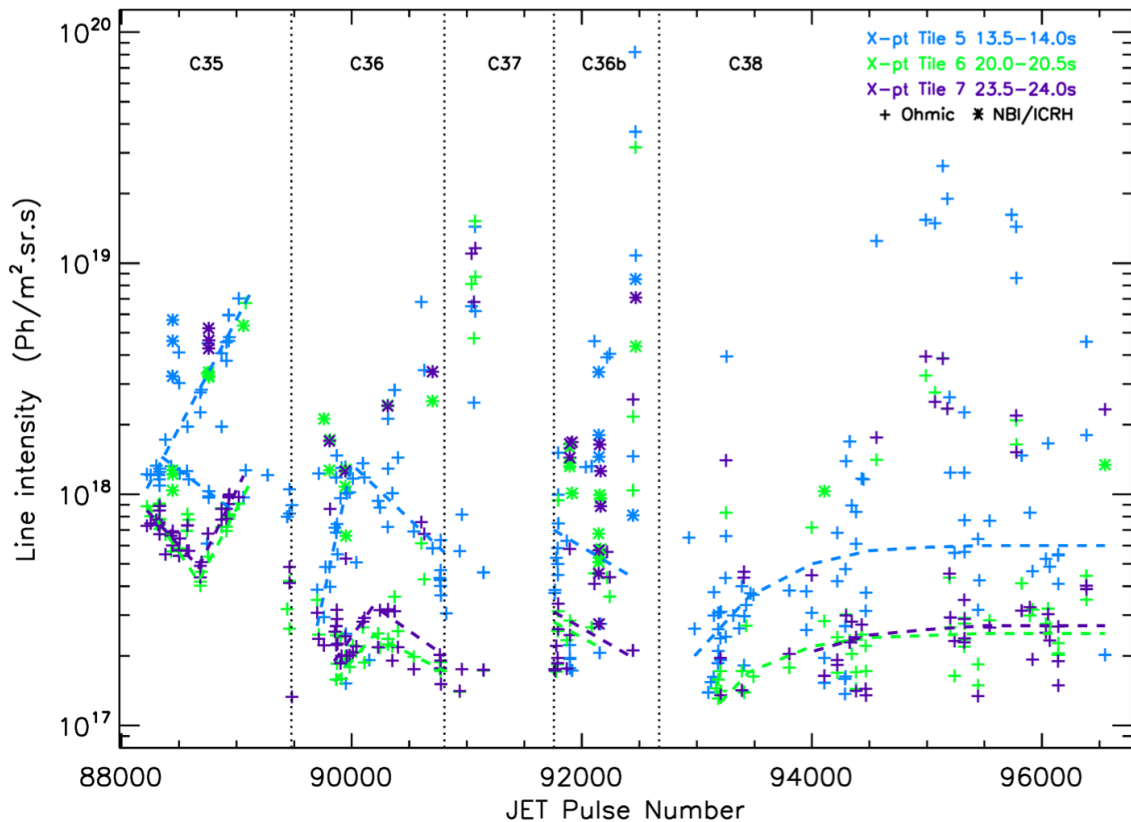
Figure 15b. X-point Ar XVI line intensities at 353.85 \text{ \AA} observed by KT7/2.
