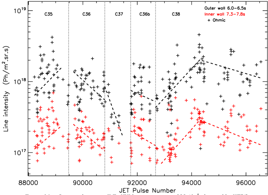
Figure 16a. Outer and inner wall Fe XVI line intensities at 335.41 \text{ \AA} observed by KT7/2.
