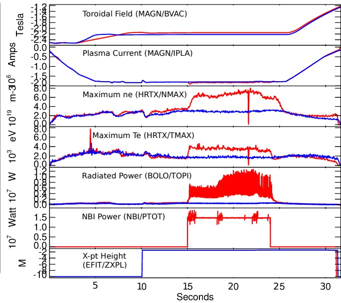
Figure 4. Plasma parameters of Ohmic DiMple pulse 91779 and with NBI, pulse 92155.
