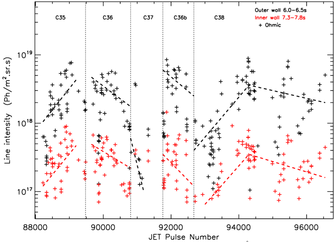
Figure 17a. Outer and inner wall Cu XIX line intensities at 273.35 \text{ \AA} observed by KT7/2.
