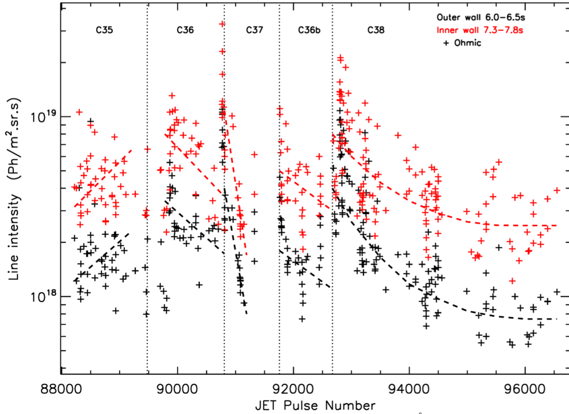
Figure 11a. Outer and inner wall O V line intensities at 629.73 \text{ \AA} observed by KT2.
