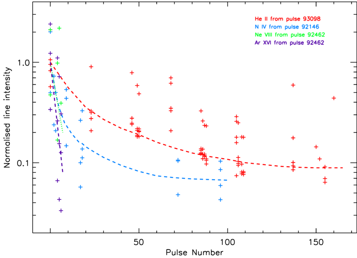
Figure 20. Decay of impurities introduced by gas-puffing
