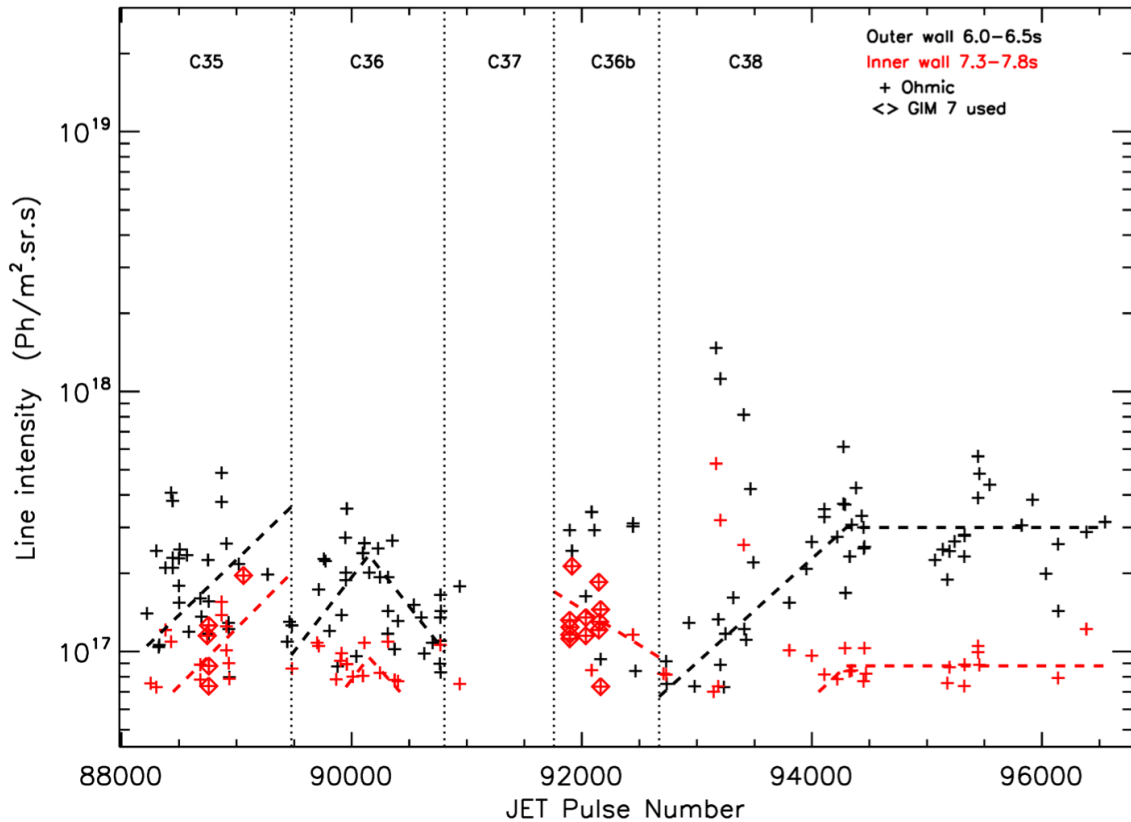
Figure 9a. Outer and inner wall C IV line intensities at 312.43 \text{ \AA} observed by KT7/2.
