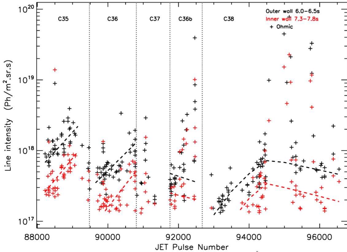
Figure 15a. Outer and inner wall Ar XVI line intensities at 353.85 \text{ \AA} observed by KT7/2.
