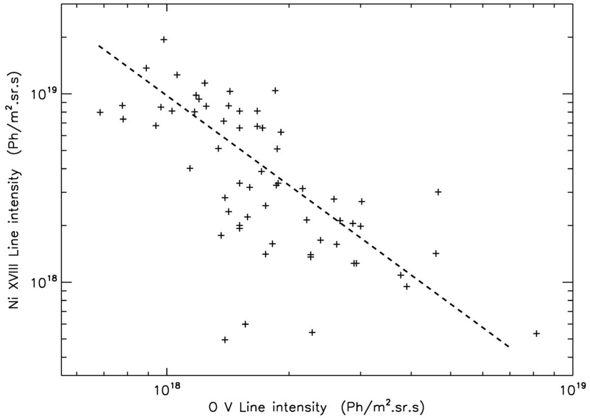
Figure 22. Outer wall O V : Ni XVIII line intensities during the C38 restart period.
