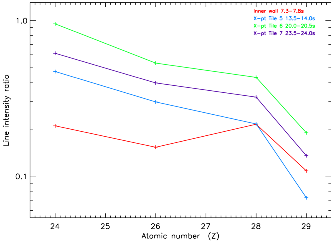
Figure 23. Mid-Z element intensities normalized to that of the Outer wall.
