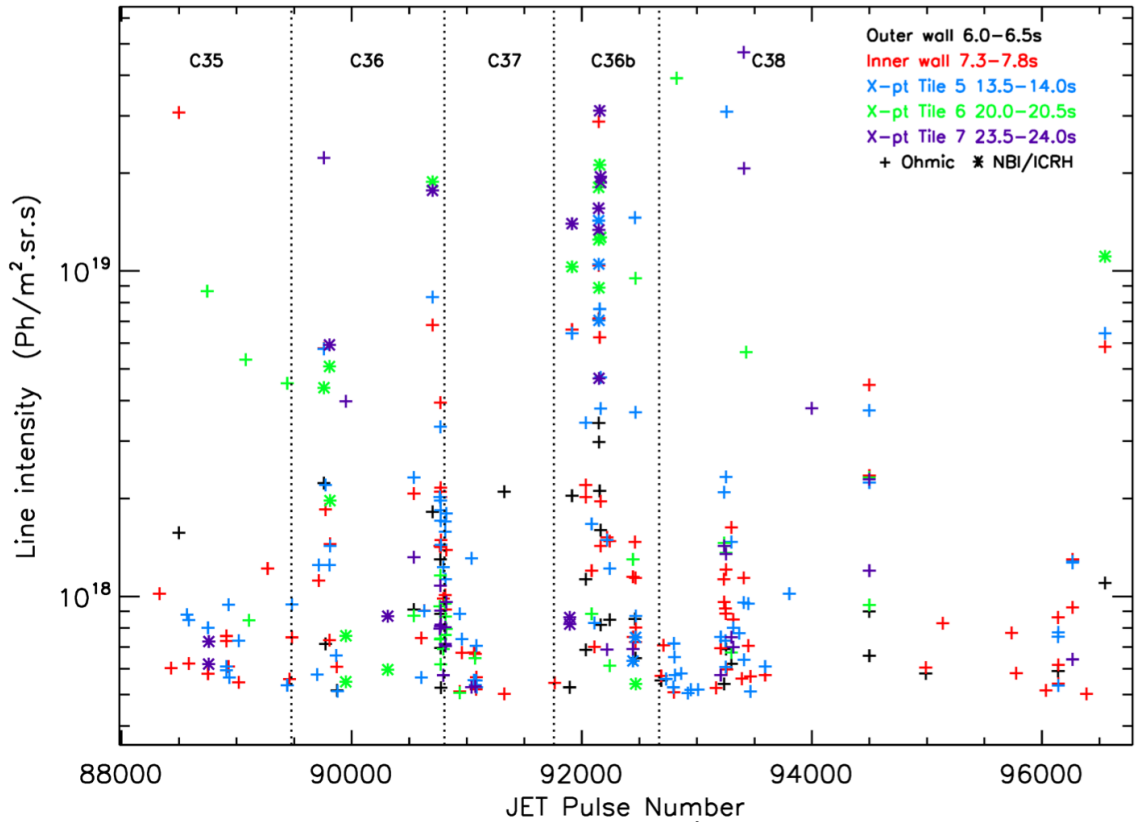
Figure 10. N IV line intensities at 923 Å observed by KT2.
