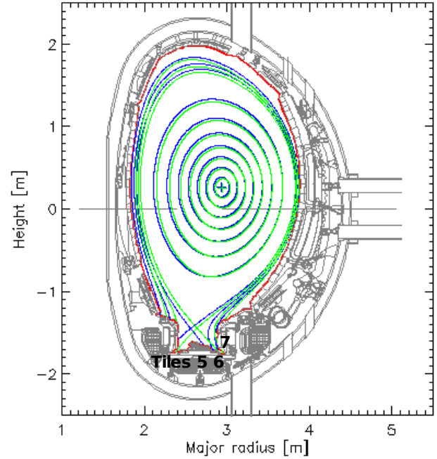
Figure 2. Magnetic configuration of the DiMple pulse 91779 X-point phases with the outer strike point on tile 5 (13.75 s) and tile 6 (20.25 s).
