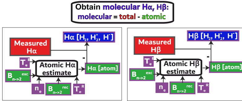
Figure 3. Schematic analysis flow chart for separating the atomic and molecular contributions from the H\alpha and H\beta emission. This represents step 2 'Obtain molecular H\alpha, H\beta ' in figure 2.
