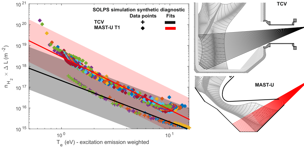
Figure 15. Relation between the excitation Balmer line emission weighted temperature T_e^E and g_{H_2}(T_e^E) \equiv \frac{B_{3 \rightarrow 2}^{H_2}}{n_e P E C_{3 \rightarrow 2}^{H_2}(n_e, T_e^E)} \approx n_{H_2} \times \Delta L (where n_e is the synthetic Stark density). Each colour corresponds to a different simulation. Fits through each of the data sets are shown. The TCV data set consists out of 5 simulations [37] (density scan) (26 lines of sight) while the MAST-U data set consists out of 35 simulations [38] (density scan and N_2 seeded) with 20 lines of sight. The corresponding SOLPS grid cells and spectroscopy lines of sight for MAST-U and TCV are also shown.
