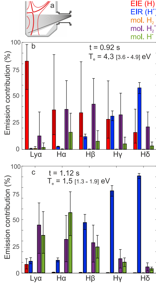
Figure 14. A schematic illustration of the divertor geometry and line of sight is shown (a). A bar-chart of the contributions (%) of various processes is shown (electron-impact excitation 'EIE ( H )', electron-ion recombination 'EIR ( H^+ )', plasma-molecule interaction ('mol.') with H_2 , H_2^+ and H^- for various hydrogenic series lines at two different times for a chord close to the target together with indicated estimated electron temperature ranges (b,c).
