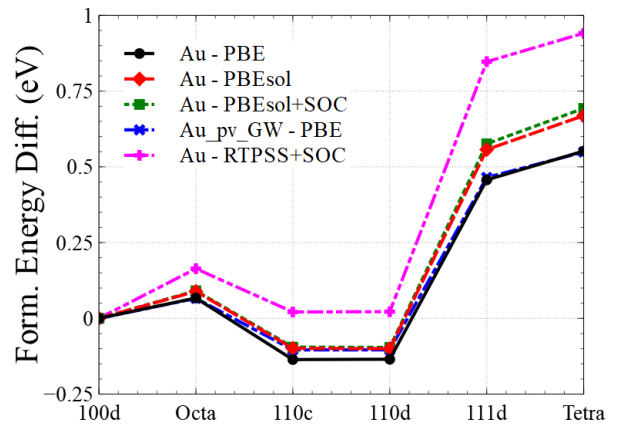
FIG. 9. Formation energies of various self-interstitial atom (SIA) defect configurations in Au. The energy of a \langle 100 \rangle dumbbell is used as a reference, and the curves show the difference between the energy of a given defect configuration and that of a \langle 100 \rangle dumbbell.
