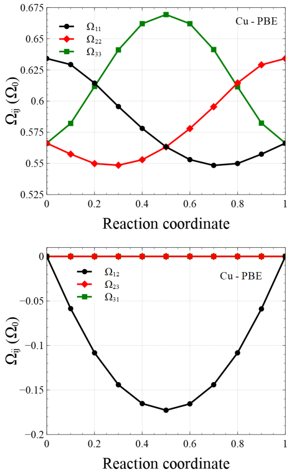
FIG. 24. Variation of elements of the relaxation volume tensor of a \langle 100 \rangle dumbbell in Cu along the migration pathway from the [100] to the [010] configuration.
