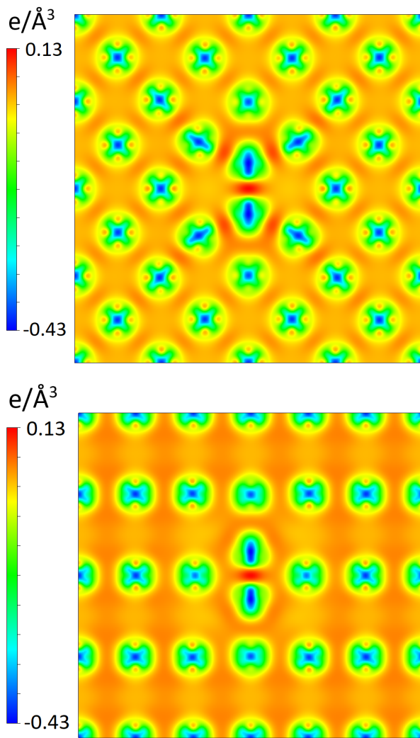
FIG. 20. Two-dimensional plots of electron charge density difference in nickel computed for a \langle 100 \rangle dumbbell configuration in the (top) (010) and (bottom) (011) planes.
