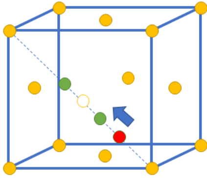
FIG. 18. Schematic illustration of one-dimensional migration of a \langle 110 \rangle crowdion / dumbbell in an FCC crystal.
