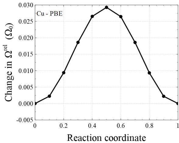
FIG. 25. Variation of the relaxation volume of a \langle 100 \rangle dumbbell in Cu along the migration pathway.
