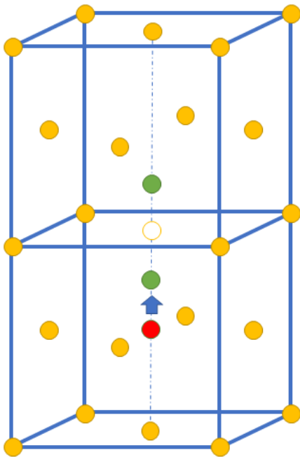
FIG. 17. Schematic illustration of the one-dimensional pathway of migration of an octahedral site interstitial defect in an FCC crystal.
