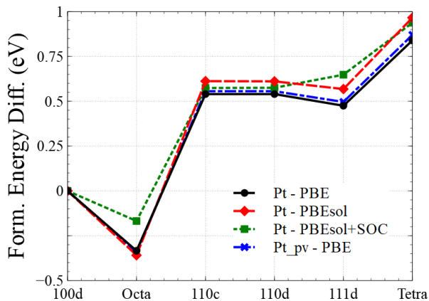
FIG. 8. Formation energies of various self-interstitial atom (SIA) defect configurations in Pt. The energy of a \langle 100 \rangle dumbbell is used as a reference, and the curves show the difference between the energy of a given defect configuration and that of a \langle 100 \rangle dumbbell.
