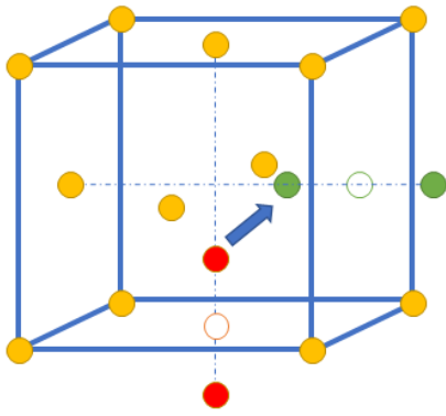
FIG. 16. Schematic illustration of the three-dimensional translation-rotation pathway of migration of a \langle 100 \rangle dumbbell from a [100] configuration to a [010] configuration in an FCC crystal.
