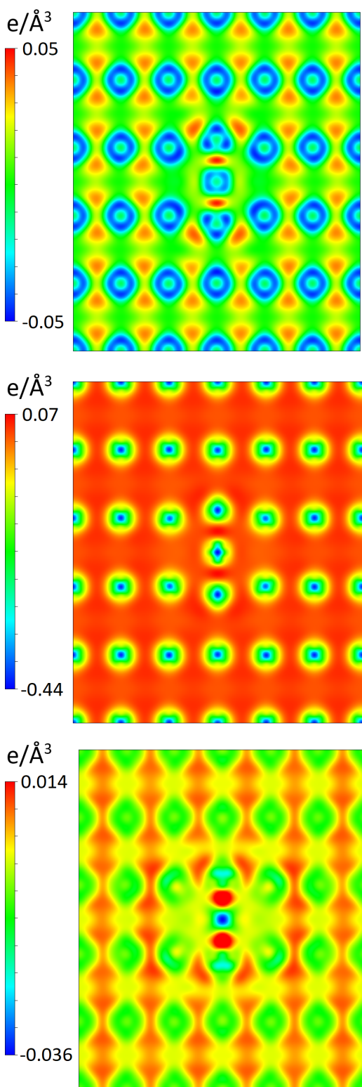
FIG. 15. Two-dimensional plots of electron charge density difference in Al (Top), Cu (middle), and Pb (Bottom), computed for an octahedral site interstitial configuration in the (011) plane.
