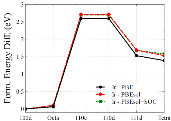
FIG. 7. Formation energies of various self-interstitial atom (SIA) defect configurations in Ir. The energy of a \langle 100 \rangle dumbbell is used as a reference, and the curves show the difference between the energy of a given defect configuration and that of a \langle 100 \rangle dumbbell.
