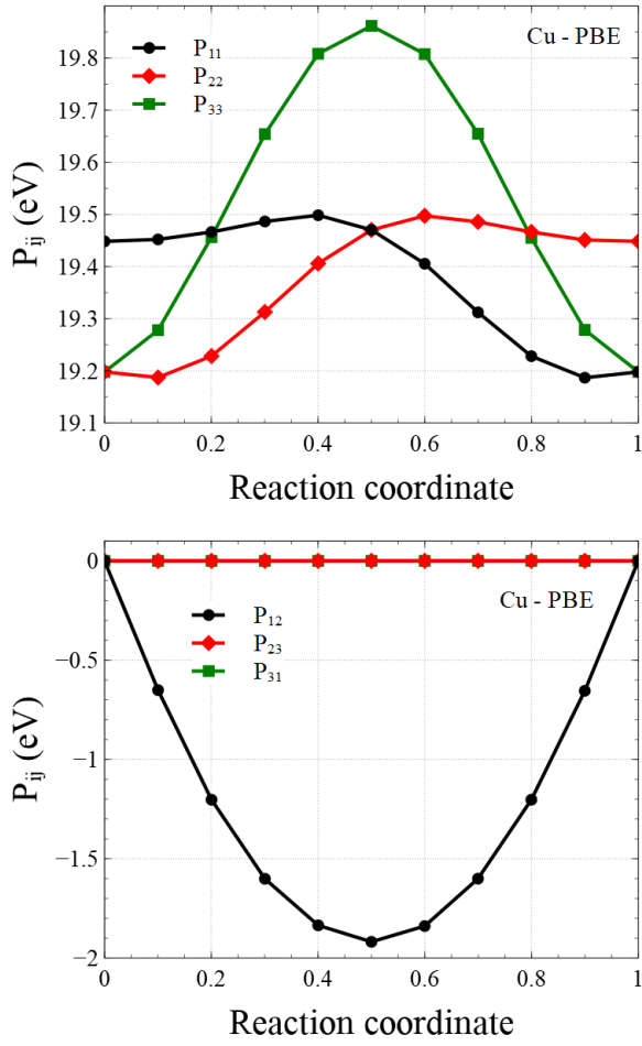
FIG. 23. Variation of elements of elastic dipole tensor of a \langle 100 \rangle dumbbell in Cu along the migration pathway from the [100] to the [010] configuration.
