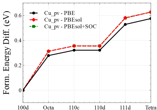
FIG. 4. Formation energies of various self-interstitial atom (SIA) defect configurations in Cu pV . The energy of a \langle 100 \rangle dumbbell is used as a reference, and the curves show the difference between the energy of a given defect configuration and that of a \langle 100 \rangle dumbbell.
