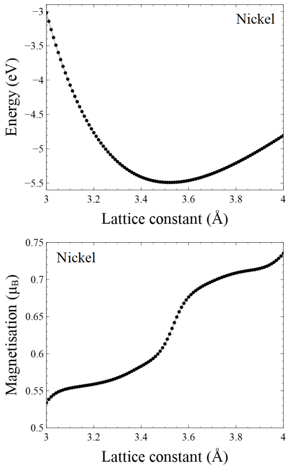
FIG. 21. Energy and magnetic moment of a nickel atom plotted as a function of the FCC lattice constant in a perfect crystal structure.
