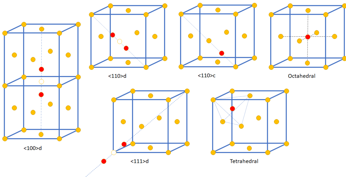
FIG. 1. Schematic sketches of self-interstitial atom defects in face-centred cubic metals. In all the cases illustrated in this figure, the simulation cell contains one extra atom, and hence each configuration represents a single-atom SIA defect. All the atoms shown in the sketches are identical, and colours highlight the symmetry of a particular defect structure. Empty spheres, where appropriate, indicate positions of unoccupied ideal lattice sites. Letters d and c refer to a dumbbell or a crowdion configuration.
