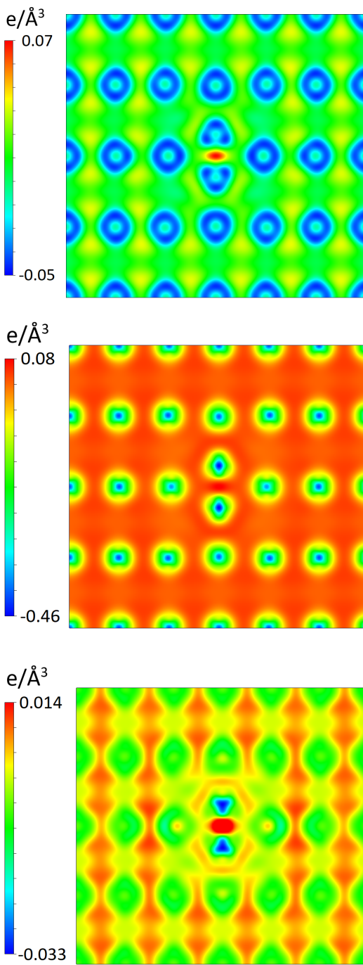
FIG. 13. Two-dimensional plots of the electron charge density difference in Al (Top), Cu (middle), and Pb (Bottom), computed for a \langle 100 \rangle dumbbell configuration in the (011) plane.
