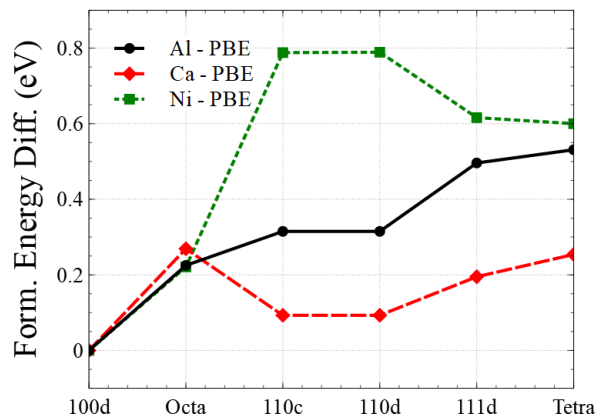
FIG. 2. Formation energies of various self-interstitial atom (SIA) defect configurations in Al, Ca, and Ni. In each case, the energy of a \langle 100 \rangle dumbbell is used as a reference, and the curves show the difference between the energy of a given defect configuration and that of a \langle 100 \rangle dumbbell.
