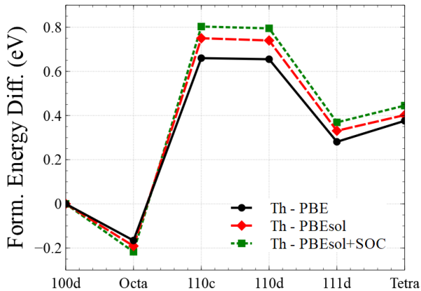
FIG. 11. Formation energies of various self-interstitial atom (SIA) defect configurations in Th. The energy of a \langle 100 \rangle dumbbell is used as a reference, and the curves show the difference between the energy of a given defect configuration and that of a \langle 100 \rangle dumbbell.
