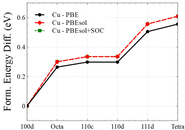
FIG. 3. Formation energies of various self-interstitial atom (SIA) defect configurations in Cu. The energy of a \langle 100 \rangle dumbbell is used as a reference, and the curves show the difference between the energy of a given defect configuration and that of a \langle 100 \rangle dumbbell.
