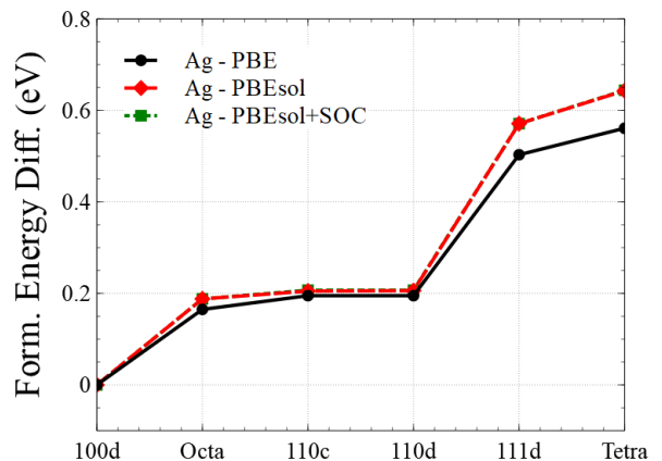
FIG. 6. Formation energies of various self-interstitial atom (SIA) defect configurations in Ag. The energy of a \langle 100 \rangle dumbbell is used as a reference, and the curves show the difference between the energy of a given defect configuration and that of a \langle 100 \rangle dumbbell.
