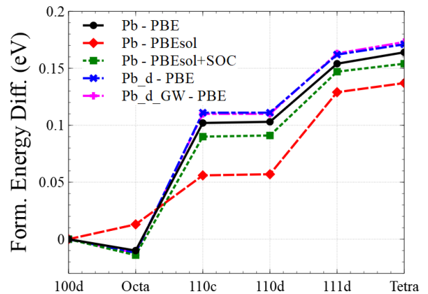
FIG. 10. Formation energies of various self-interstitial atom (SIA) defect configurations in Pb. The energy of a \langle 100 \rangle dumbbell is used as a reference, and the curves show the difference between the energy of a given defect configuration and that of a \langle 100 \rangle dumbbell.
