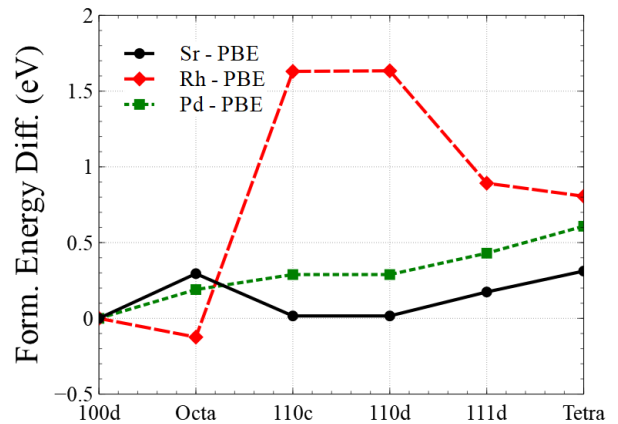
FIG. 5. Formation energies of various self-interstitial atom (SIA) defect configurations in Sr, Rh, and Pd. The energy of a \langle 100 \rangle dumbbell is used as a reference, and the curves show the difference between the energy of a given defect configuration and that of a \langle 100 \rangle dumbbell.
