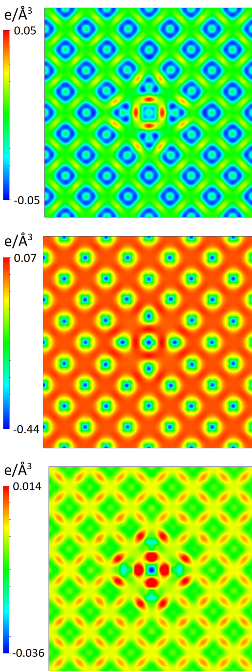
FIG. 14. Two-dimensional plots of electron charge density difference in Al (Top), Cu (middle), and Pb (Bottom), computed for an octahedral site interstitial configuration in the (010) plane.
