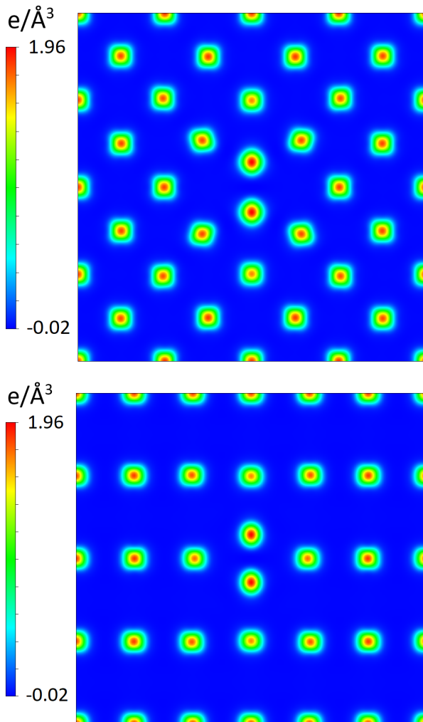
FIG. 19. Two-dimensional plots of magnetization density in nickel, computed for a \langle 100 \rangle dumbbell configuration in the (top) (010) and (bottom) (011) planes.
