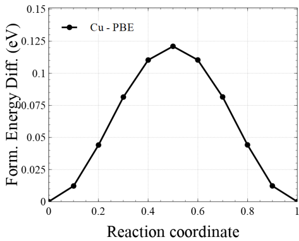
FIG. 22. Variation of the formation energy of a \langle 100 \rangle dumbbell in Cu along the migration pathway of the defect.
