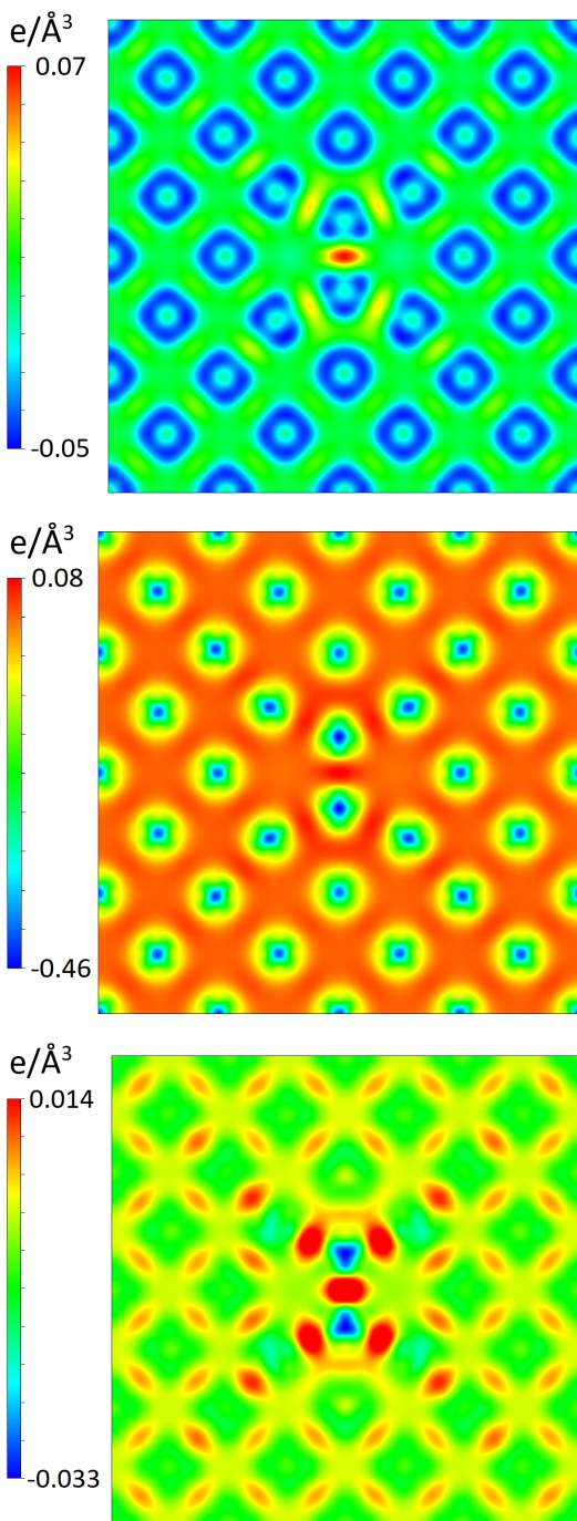
FIG. 12. Two-dimensional plots of the electron charge density difference in Al (Top), Cu (middle), and Pb (Bottom), computed for a \langle 100 \rangle dumbbell configuration in the (010) plane. Electron charge density difference is defined as the fully convergent electron density derived from ab initio simulations minus the superposition of atomic charge densities.
