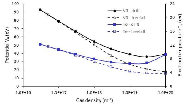
FIG. 2. (Colour online) The potential V_0 and the plasma electron temperature T_e for a nominal 120kV, 60A deuterium beam with radius A=0.1 m as a function of the
