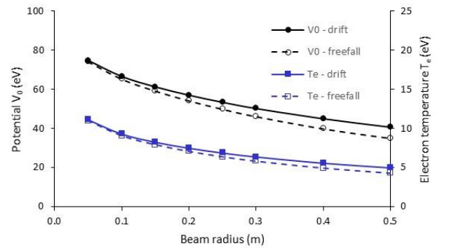
FIG. 5. (Colour online) The dependence of the potential V_0 and the electron temperature T_e on beam radius for the nominal 120kV, 60A beam with a background gas density of 3 \times 10^{17} \text{m}^{-3} for the two models.
