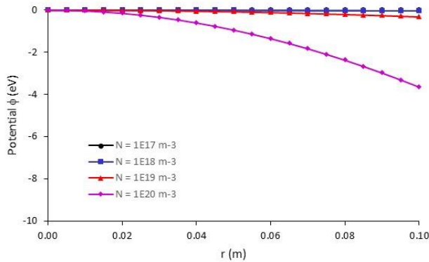
FIG. 6. (Colour online) The radial potential dependence within the beam for a 120kV, 60A beam at different background gas densities for the drift model with a beam radius A = 0.1\text{m} .
