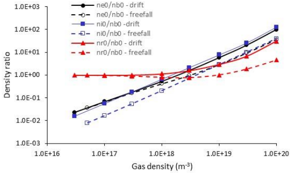
FIG. 3. (Colour online) The axial densities of the plasma electrons ( n_{e0}/n_{b0} ), slow positive ions ( n_{i0}/n_{b0} ) and the fast electrons ( n_{r0}/n_{b0} ) relative to the beam ion density ( n_{b0} ) for the nominal 120kV, 60A beam with radius A=0.1\text{m} .
