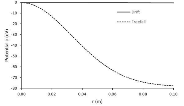
FIG. 7. The radial potential dependences within the beam for a 120kV, 60A beam at a background gas density of 10^{17}\text{ m}^{-3} with a beam radius A = 0.1\text{m} for both the drift and freefall models.
