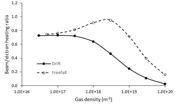
FIG. 4. The ratio of the beam and fast electron heating contributions to the plasma electrons for the nominal 120kV, 60A beam with radius A=0.1\text{m} for the two models.
