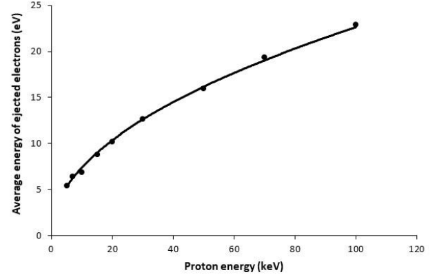
FIG. 1. The average energy of ejected electrons in H^+ + H_2 collisions.
