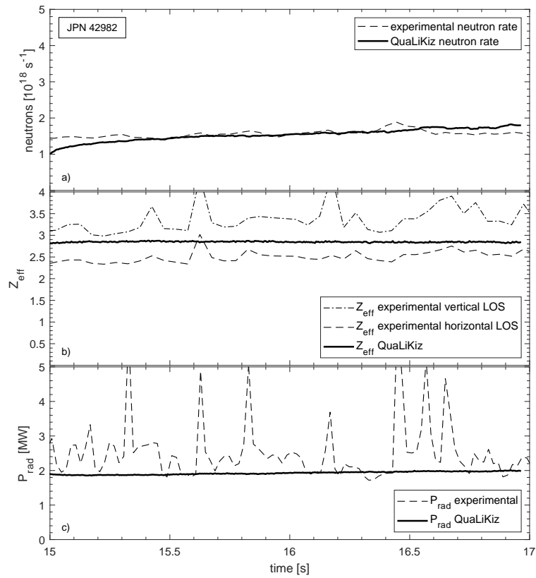
Figure 11. Comparison between experimental and modelled neutron rate (a), Z_{eff} (b) and radiated power (c) for shot 42982. Z_{eff} is inferred from Bremsstrahlung measurements along a vertical and a horizontal line of sight across the plasma and radiated power from bolometry.
