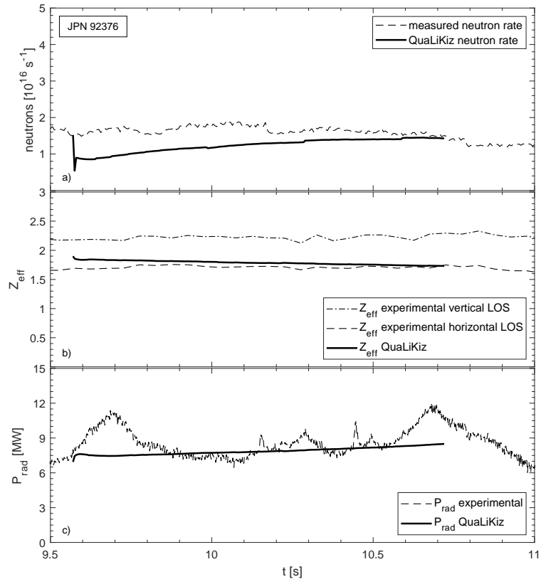
Figure 3. Comparison between experimental and modelled neutron rate (a), Z_{eff} (b) and radiated power (c) for shot 92376. Z_{eff} is inferred from Bremsstrahlung measurements along a vertical and a horizontal line of sight across the plasma and radiated power from bolometry.
