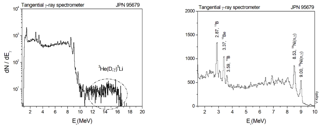
Figure 5. Gamma-ray spectrum recorded by the \text{LaBr}_3 detector in discharge #95679: (a) – a log-scale spectrum displays the detected 17-MeV gammas and (b) – a linear-scale zoomed spectrum clearly showing the gammas from the ^9\text{Be}(D,n\gamma)^{10}\text{B} and ^9\text{Be}(D,p\gamma)^{10}\text{Be} nuclear reactions.
