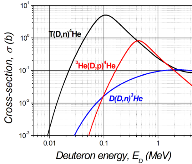
Figure 1. The cross-sections of D - D , D - ^3\text{He} and D - T reactions [4] as a function of the energy of fast D -ions.
