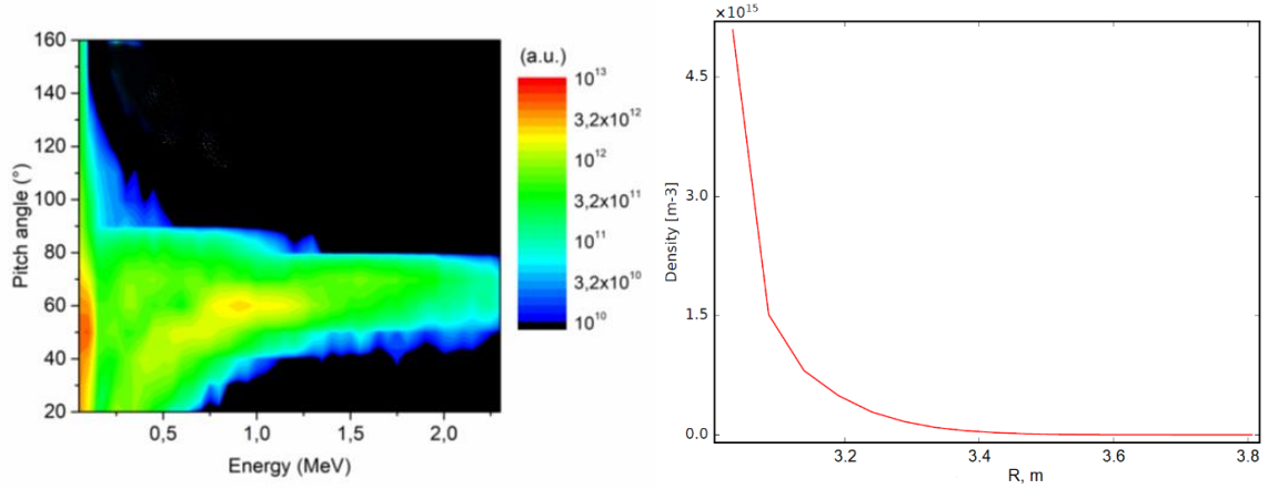
Figure 7. a – Pitch-angle versus energy distribution of the D-ions from TRANSP in JET discharge #95679; b – The radial profile of the alpha-particle density after slowing-down averaged over time interval 10.9 – 11.0 s.
