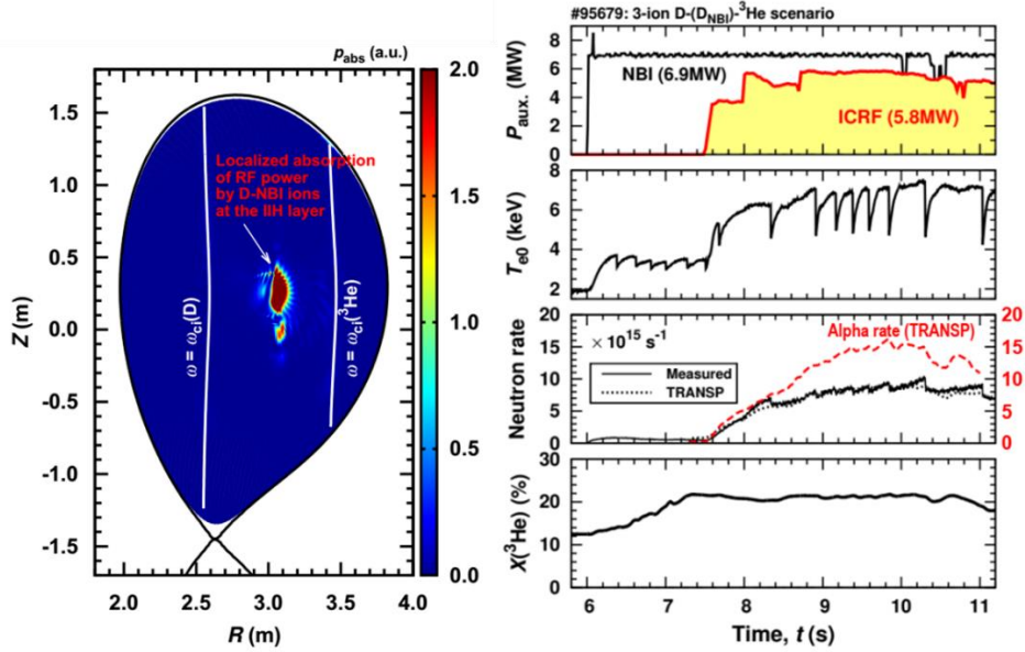
Figure 2. (a) – The poloidal cross-section of the JET tokamak showing the off-axis location of the cyclotron resonances of ^3\text{He} - and D -ions and the core absorption of RF power by fast D -NBI ions in the close vicinity of the IH layer, as calculated with the TORIC code; (b) – An overview of JET pulse #95679. The panels show the auxiliary heating power from NBI and ICRH, the central electron temperature, T_{\text{e0}} , the measured D - D neutron rate (black solid line) vs. the TRANSP simulation (black dotted line) and the TRANSP-simulated D - ^3\text{He} fusion alpha-particle rate (red dashed line). The bottom panel shows the ^3\text{He} concentration controlled by the real-time feedback system.
