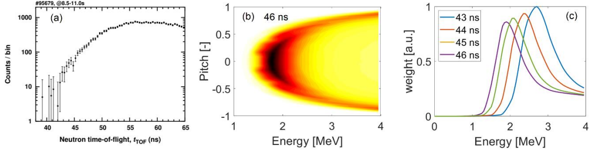
Figure 8. a – Neutron time-of-flight spectrum recorded in discharge #95679 by TOFOR; b – TOFOR weight function calculated in (E_D, \lambda) -space for the time-of-flight 46 ns; c – TOFOR weight functions integrated over pitch for several time-of-flights.
