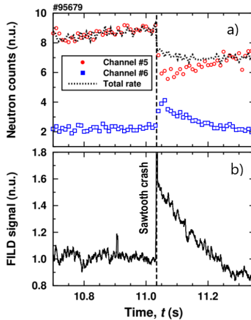
Figure 18. (a) – Time evolution of the total neutron rate and rates in the central and outer channels of the neutron camera; (b) – FILD alpha-particle losses with E_\alpha > 4.5 MeV before and after the monster sawtooth crash at t = 11.03 s.
