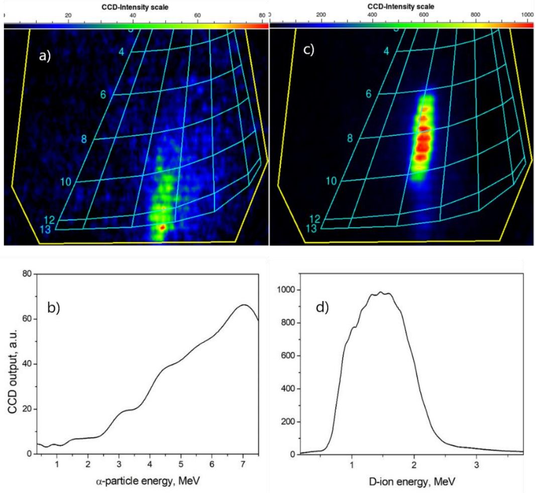
Figure 13. FILD data obtained in discharge #94698 at the monster sawtooth at 10.53s: (a) – Footprint of losses recorded before the sawtooth crash; (b) – Losses at pitch-angle \theta = 57.5^\circ versus alpha-particle energy recorded before the sawtooth crash; (c) – Footprint of losses recorded during the sawtooth crash; (d) – Losses at pitch-angle \theta = 52.75^\circ versus D -ion energy recorded during the sawtooth crash.
