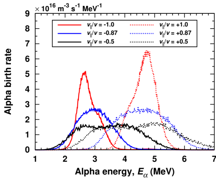
Figure 14. The birth energy spectra of the D - ^3\text{He} fusion-born alpha-particles obtained with the code GENESIS using as input the distribution function of ICRF-accelerated D -ions for discharge #95679 calculated with TRANSP (see figure 7).
