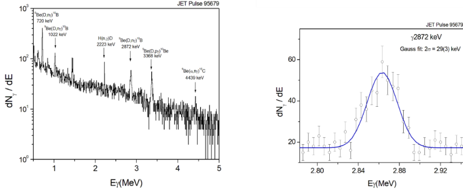
Figure 6. (a) – Gamma-ray spectrum recorded by HpGe-detector for t = 8.5-11.5 s of JET discharge #95679; (b) – Experimental data together with the best Gaussian fit for the Doppler broadened gamma-ray line 2872 keV from the {}^9\text{Be}(D,n){}^{10}\text{B} reaction.
