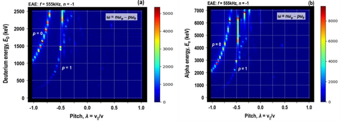
Figure 19. Resonance maps for observed n = -1 EAE ( f_{\text{EAE}} \approx 555 kHz as in discharge #95679) showing the resonances for p = 0, +1 for (a) D -ions and (b) alpha-particles. The computations have been carried out using the HAGIS and MISHKA codes for a fixed mode amplitude \delta B/B = 10^{-5} . Weak higher-order wave-particle resonances for p = +2, +3 \dots are also visible, but only at negative pitches and high ion energies.
