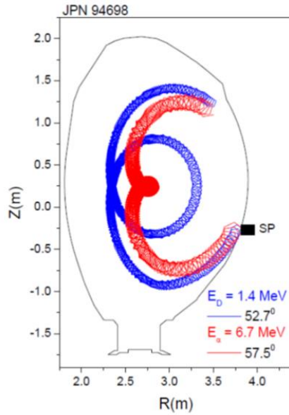
Figure 15. Orbits of lost fast ions calculated backward-in-time from the FILD scintillator plate: red line – alpha-particle orbit with E_\alpha = 6.7 MeV and \theta = 57.5^\circ ; blue line – D -ion orbit with E_D = 1.4 MeV and \theta = 52.7^\circ ; these parameters are related to the footprints presented in figure 12.
