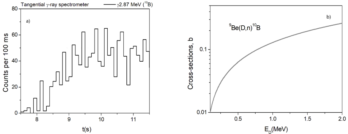
Figure 9. (a) – Waveform of the peak 2.87 MeV; (b) – Cross-section of the {}^9\text{Be}(D, n){}^{10}\text{B} reaction.
