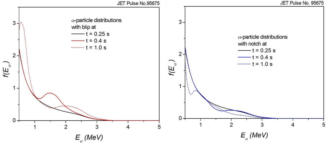
Figure 20. Temporal evolution of the f_\alpha(E) function for a blip and a notch set at the moment of the sawtooth crash ( t = 0 s) in discharge #95675; slowing-down of alpha-particles were calculated with the birth spectrum for v_{\parallel}/v = -1 (see figure 13).
