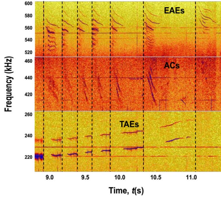
Figure 16. Magnetic spectrograms demonstrate fast-ion driven Alfvén eigenmodes observed in JET discharge #95679; vertical dashed lines denote the timing of the sawtooth crashes.
