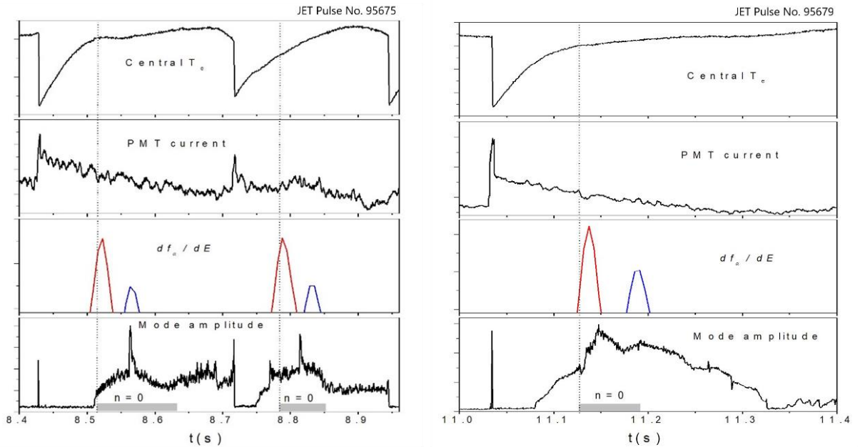
Figure 22. Comparison of the time evolution of T_{e0} , FILD PMT#11 currents, \partial f_\alpha / \partial E (red – blips, blue – notches) and mode amplitudes (grey bars – periods where the n=0 mode is present) during sawteeth in discharges #95675 and #95679 (see figure 17); dotted lines mark the onset of the n=0 AEs.
