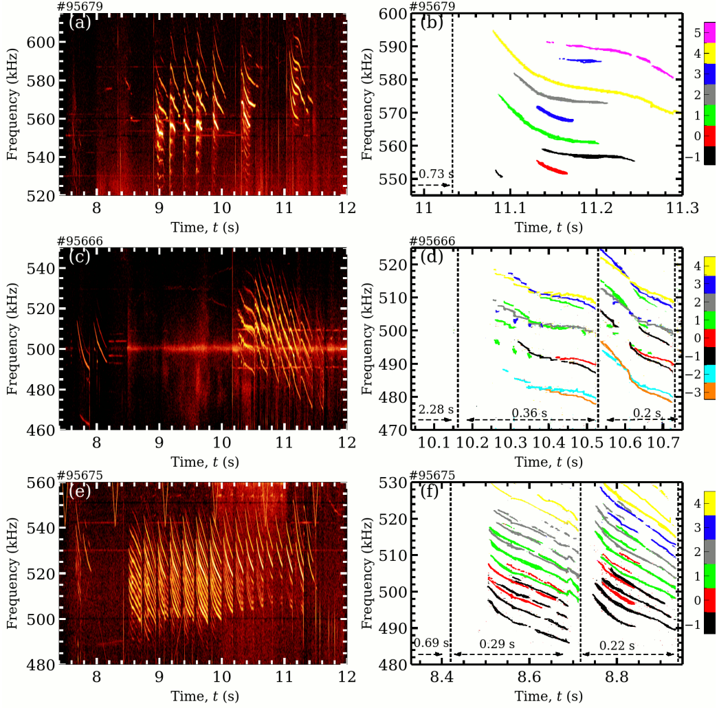
Figure 17. Magnetic spectrograms together with toroidal mode numbers for AEs detected in discharges #95675 and #95679.
