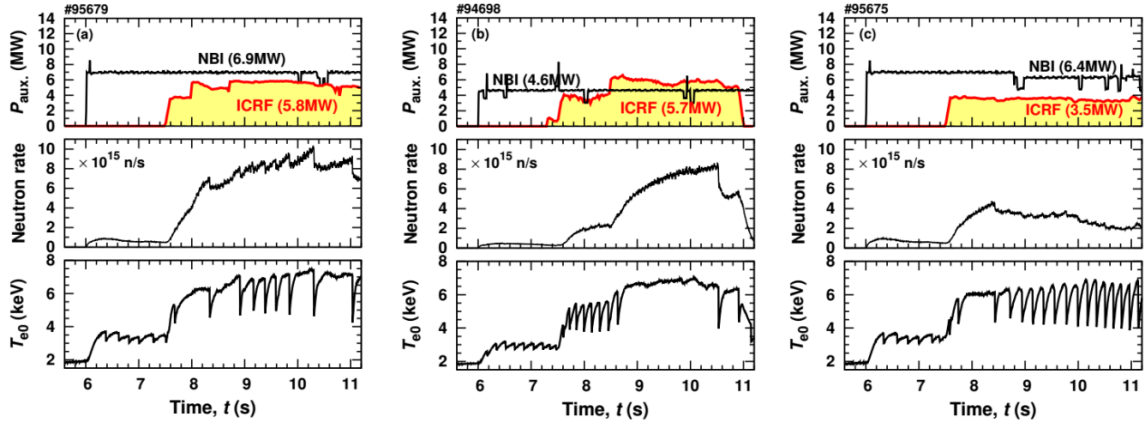
Figure 4. Overview of three pulses in mixed D - ^3\text{He} plasmas on JET with different sawtooth characteristics obtained by varying P_{\text{ICRF}} and P_{\text{NBI}} . The panels from top to bottom show the NBI and ICRF power, the neutron rate and the central electron temperature. Various sawtooth behaviours were observed during the combined NBI+ICRF heating phase: (a) in pulse #95679: short-period sawteeth during t = 8.6 - 9.7 s; (b) in pulse #94698: monster sawtooth during t = 8.63 - 10.53 s; (c) in pulse #95675: short-period sawteeth during t = 8.8 - 11.0 s.
