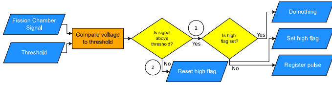
FIG. 2: Flow chart of the pulse detection algorithm.
