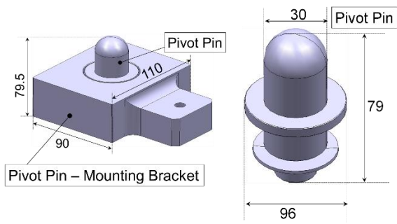
Figure 33 Left: ‘Pivot Pin-Mounting Bracket’ assembly which is attached to the ‘Baseplate’ (see Figure 32). Right: ‘Pivot Pin’ assembly. Dimension in millimetres.
