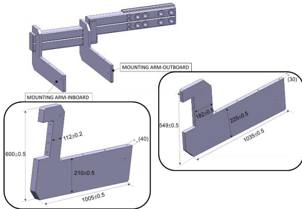
Figure 43 Model and dimensions (mm) of the mounting arms.
