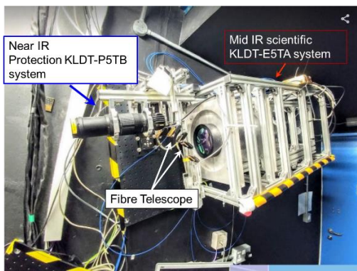
Figure 53 Photo showing DIR viewing systems inside 'Middle Lab'.
