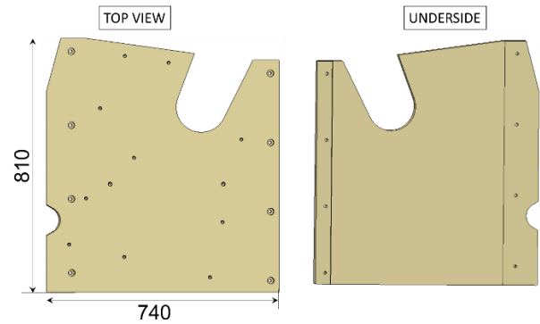
Figure 44 Top and underside views of 'M4 Mirror Support Plate' assembly with key dimensions in millimetres.
