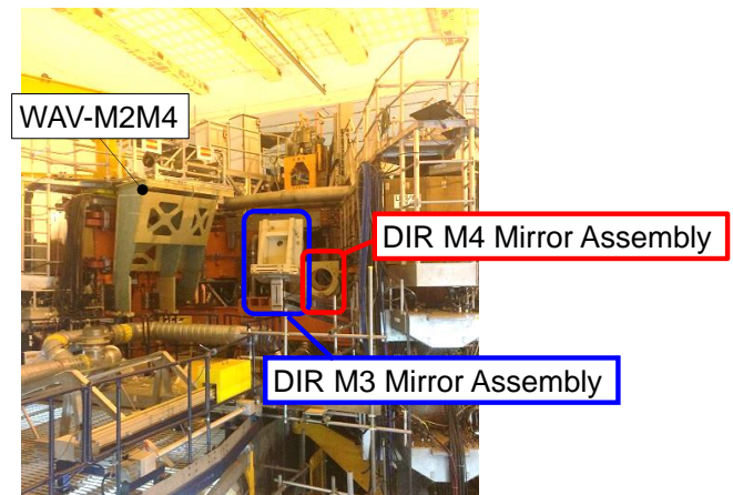
Figure 19 Photo of the installed M3 and M4 mirror assemblies.
