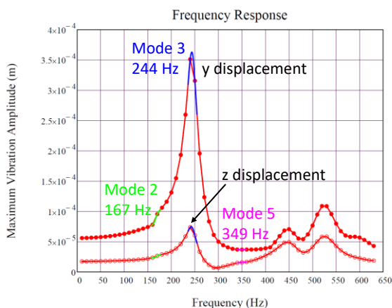
Figure 25 Harmonic analysis of the DIR-L1-M1-M2 assembly depicting the different modes as a function of amplitude in metres for mirror M2 (see reference [20]).
