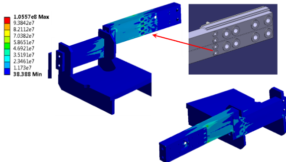
Figure 46 Model showing static structural stress levels in MPa as a function of colour.
