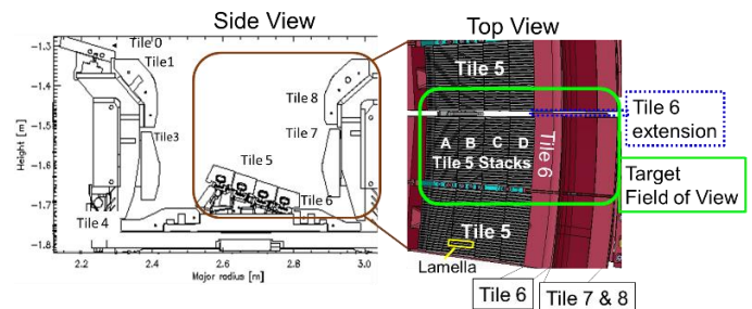
Figure 1 Left: Side view of divertor region with a brown boxed area for target field of view. Right: Top view of divertor region from CAD model with green boxed area to show target field of view.
