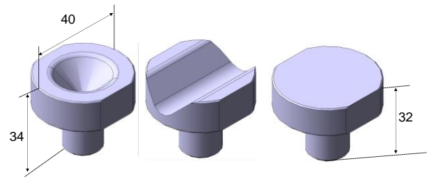
Figure 21 Kinematic receiving contact parts or kinematic 'feet': Cone (left), Vee (middle) and Flat (right).
