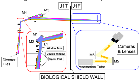
Figure 8 DIR Mirror relay showing the Zemax ray tracing (pyrometers are not shown).
