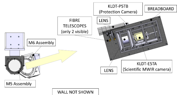
Figure 50 Schematic of the DIR assemblies in the ‘Middle Lab’.
