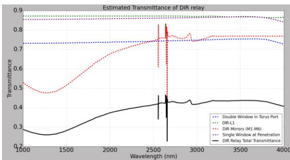
Figure 11 Estimated DIR relay Transmittance in the black trace. Dashed lines represent the estimated transmission of the main components: double window in Torus port (blue), L1 (green), single window at penetration (magenta) and estimated reflectivity from DIR mirrors (red).
