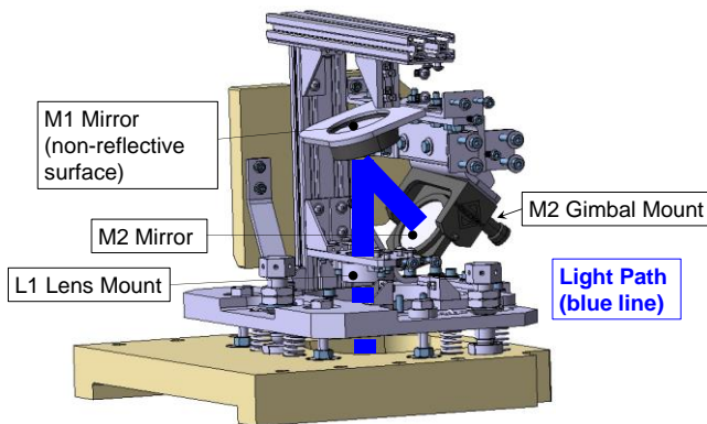
Figure 23 Side view of L1, M1 and M2 including the light path (thick blue line) with one of the side plates removed.
