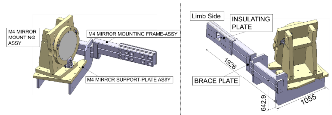
Figure 41 Side and rear views of the DIR M4 assembly.
