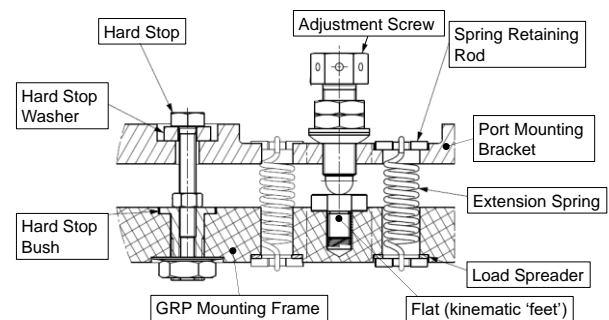
Figure 22 Cross section as example of the adjustment screws. This figure shows specifically the 'Flat' kinematic feet.
