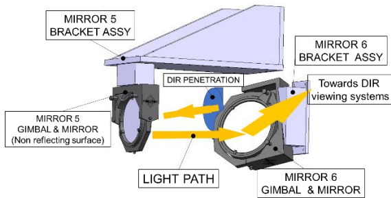
Figure 49 DIR M5 and DIR M6 mirror assemblies located outside the Torus Hall. The outside of the biological shield wall is not shown. The yellow arrows represent the light path.
