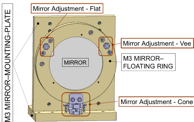
Figure 31 Front view of the M3 Mirror mounting assembly.
