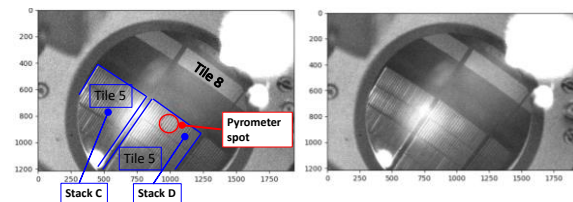
Figure 7 Pyrometer back-illuminated spot-on stack D on Tile 5 with (left) and without (right) labels for better contrast.
