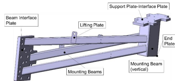
Figure 30 Key components of the M3 'Mounting Arm' assembly.
