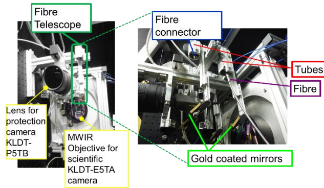
Figure 17 Photo showing the location of the fibre telescopes in between the Canon lens of the protection camera (KLDT-P5TB) and the MWIR objective for scientific KLDT-E5TA camera. Parts shown on Figure 16 are also labelled in the photo.
