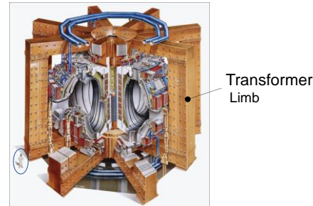
Figure 3 JET tokamak picture showing the transformer limbs. The size of the JET tokamak has been compared with to a person’s size (see reference [5]).
