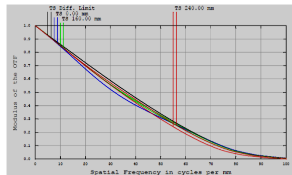
Figure 14 Modulation Transfer Function for the objective of the middle infrared divertor camera (KLDT-E5TA).
