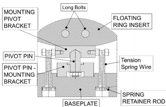
Figure 37 Cross section showing the ‘Mounting Pivot Bracket’ and ‘Pivot Pin’ within the ‘Floating Ring Insert’ and the ‘Base Plate’.
