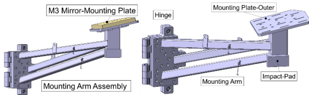
Figure 28 Left: Model depicting the mounting arm and plate assemblies. Right: Model depicting the main sub-assemblies of the 'Mounting Arm Complete' assembly.
