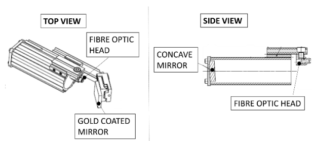
Figure 16 Key features of the fibre telescope.
