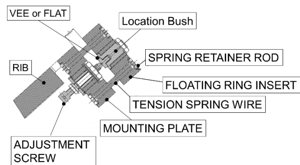
Figure 36 Top view cross section of the Vee or Flat ‘Adjustment Screw’ assembly listing the main components.
