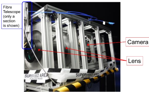
Figure 52 Photo showing the mounting frame of KLDT-E5TA inside the 'Middle Lab' and a section of one of the fibre telescopes.
