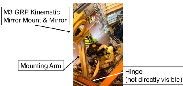
Figure 40 Photo taken from above of two operatives located on a MEWP closing the hinge and placing the DIR-M3 in the ‘closed’ position.
