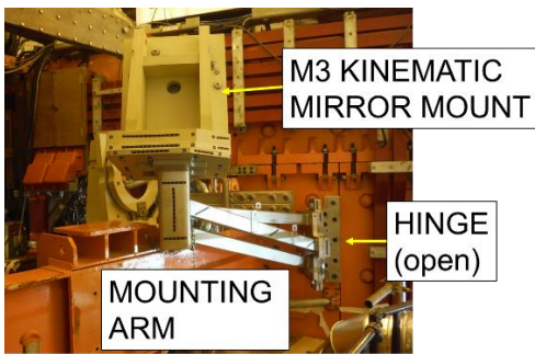
Figure 39 Rear view of the DIR-M3 after being installed with the hinge in the open position.
