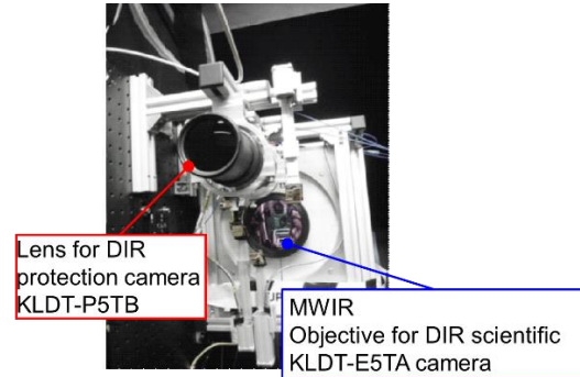
Figure 15 Positional layout of the Canon lens for the protection camera in DIR (KLDT-P5TB), the front surface of the MWIR objective for the scientific camera KLDT-E5TA and the fibre telescopes.
