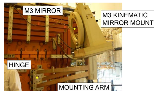
Figure 38 Side view of DIR-M3 after being installed with the hinge in the closed position.
