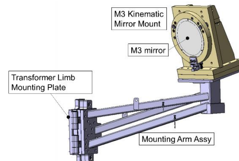
Figure 27 DIR-M3 assembly pointing the main sub-assemblies.
