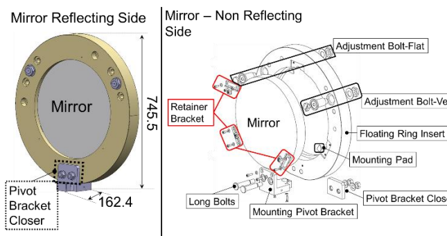
Figure 34 Left: front view of the Floating Ring assembly with dimensions in millimetres. Right: exploded view of the Floating Ring Insert assembly, mirror and other key parts mentioned in the text.
