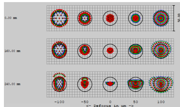
Figure 13 Through Spot Diagram for the objective of the middle infrared divertor camera KLDT-E5TA.
