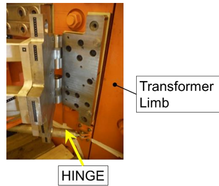
Figure 29 Photo taken during the installation of the assembly of the hinge fixed to the transformer limb. The hinge is shown in the open position.
