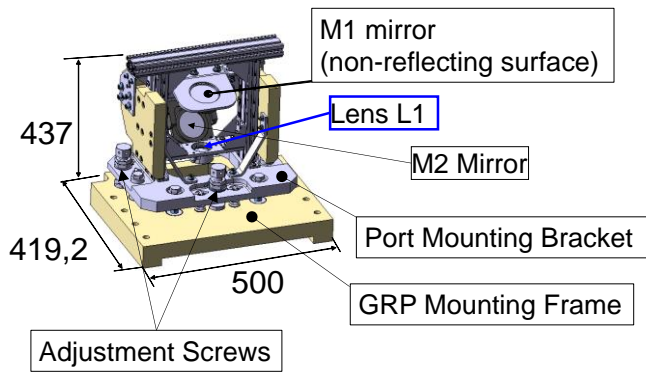
Figure 20 Front view of the DIR-L1-M1-M2 assembly noting overall dimensions in millimetres and key components.
