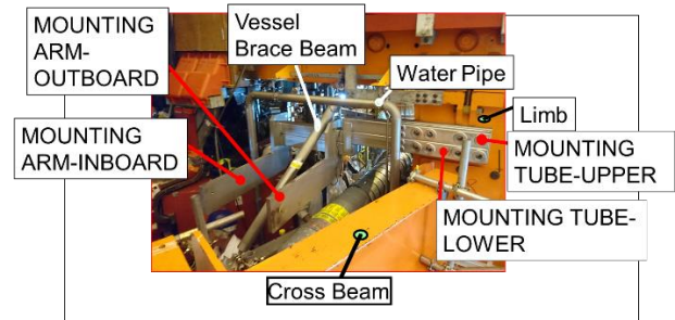
Figure 47 Photo taken after the installation of only the 'M4 Mirror Mounting Frame'.
