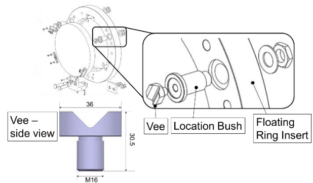
Figure 35 View of the Vee foot on its own (bottom left picture) with dimensions in millimetres and inside a close up of the Floating Ring assembly.
