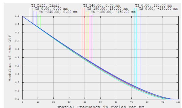
Figure 10 Modulation transfer function for DIR mirror relay.
