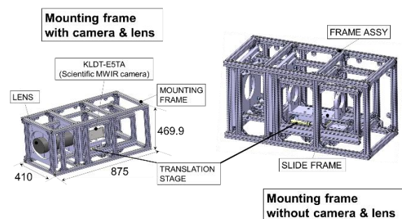
Figure 51 Mounting frame for KLDT-E5TA.
