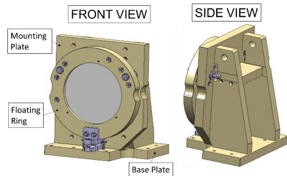
Figure 45 Front and side views of DIR-M4 Mirror Mounting.
