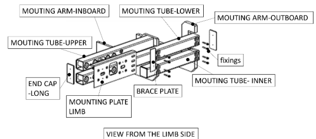
Figure 42 Exploded view of the DIR-M4 Mirror Mounting Frame assembly listing the key components.
