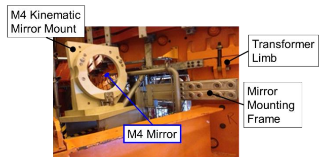
Figure 48 Photo taken after the installation of the DIR-M4 complete assembly.
