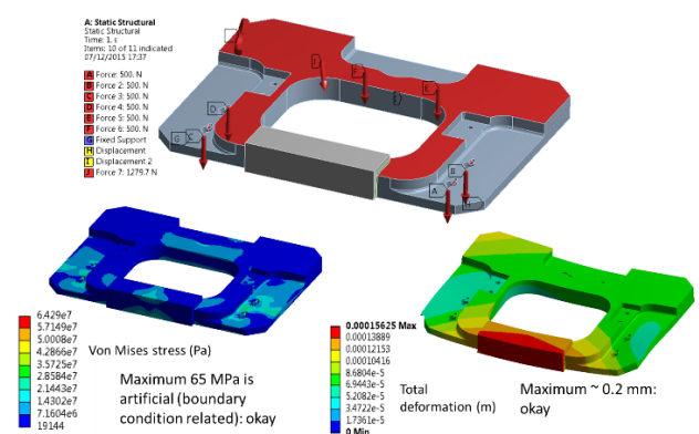
Figure 24 Analysis model showing static stresses and deformations in ‘Port Mounting Bracket’ (see reference [16]).
