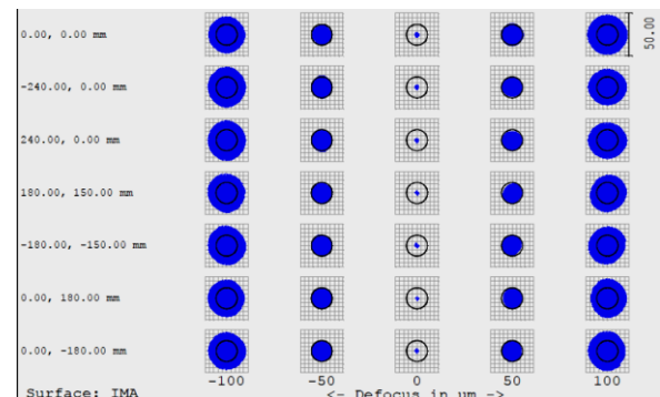
Figure 9 Through focus spot diagram for DIR mirror relay.
