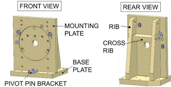
Figure 32 Front and rear view of the M3 mirror mounting listing the key parts.
