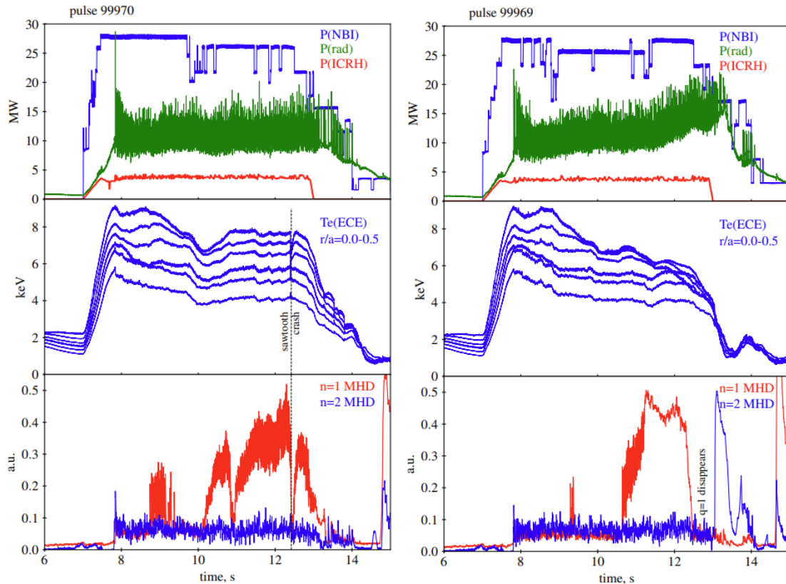
Figure 10: Examples of pulse evolution throughout the heating phase. From top to bottom: NBI, ICRH and radiated power, electron temperature (ECE) at different radii, MHD activity through Mirnov coils signal correlation for toroidal mode numbers n=1 and n=2 . Left) #99970 stationary pulse with fishbones transitioning to n=1 and sawtoothing plasma. b) #99969 core impurity accumulation causes the hollowing of Te profile, broadening of plasma current and emerging of n=2 MHD activity.
