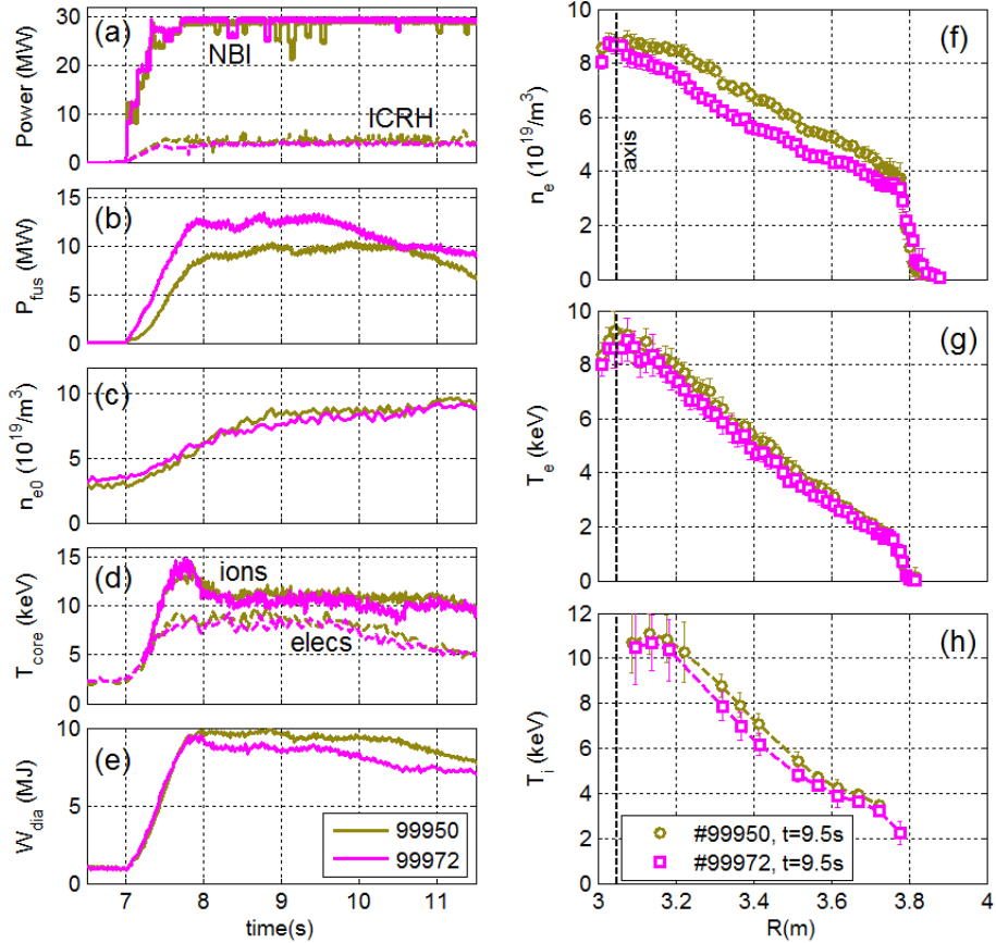
Figure 12: Comparison between 50/50 D/T (#99950 gold) and T-rich (#99972 magenta) hybrid discharges; a) NBI+ICRH heating power; b) fusion power, c) central plasma density, d) central electron (HRTS) and ion (CXRS) temperatures; e) diamagnetic stored energy; f) electron density profiles, g) electron temperature profiles, h) ion temperature profiles.
