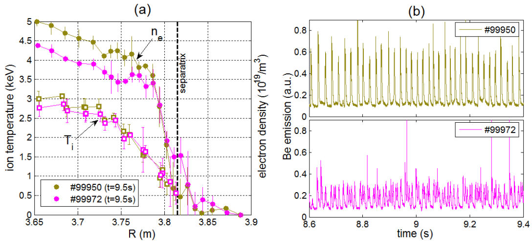
Figure 13: (a) Electron density (HRTS) and ion temperature (edge CXRS) profiles vs mid-plane plasma radius in the pedestal region for pulses #99950 (50-50 D-T type I ELM hybrid H-mode) and #99972 (T-rich hybrid H-mode with small ELMs) at t=9.5s ; The dashed line indicates the separatrix position according to EFIT; (b) Beryllium line intensity at the outer divertor (same scale) illustrating the different ELM dynamics in the two discharges.
