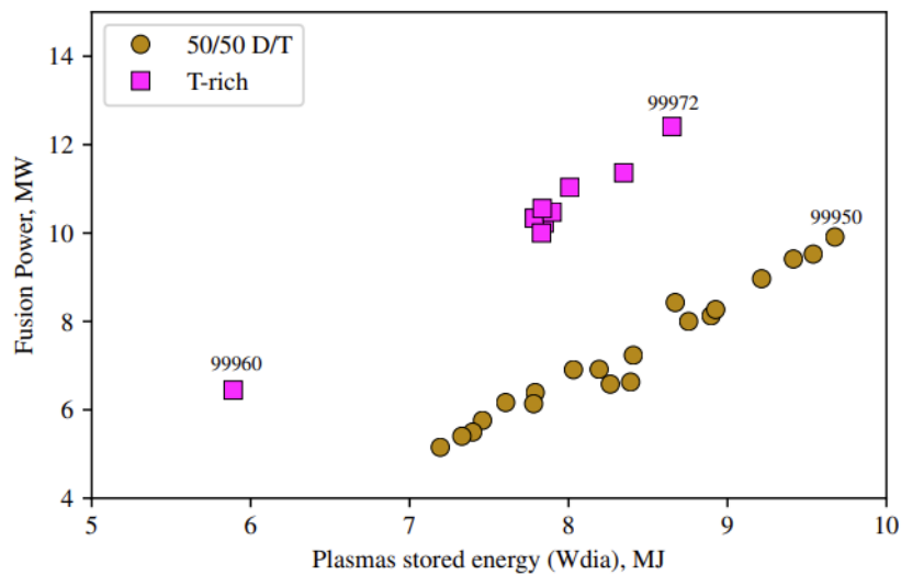
Figure 15: Generated fusion power versus plasma diamagnetic energy ( W_{dia} ) for the tritium rich pulses (magenta) and 50/50 D/T hybrid pulses (gold). The data for each pulse is averaged over the time window of t=8-10s
