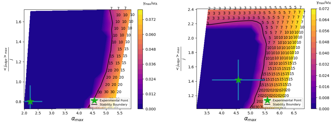
Figure 14: Left: Pedestal stability diagram of T-rich pulse #99972. Right: Pedestal stability diagram of 50/50 D/T pulse #99950 with type I ELMs
