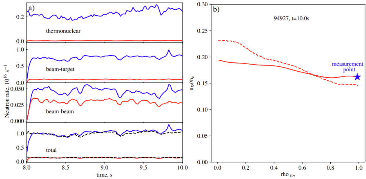
Figure 2: a) Total neutron rate and its components (thermonuclear, beam-target and beam-beam) as calculated by a TRANSP simulation and comparison with the measured neutron rate (dashed). The simulations are done for pure deuterium plasmas (94925, blue) and hydrogen-rich plasmas (94927, red) b) Deuterium concentration profile of the hydrogen-rich plasma discharge, solid line - the input to the TRANSP simulation with neutron rate matching the experimental value, dashed line – results of predictive JINTRAC-Qualikiz simulation (see section 7)
