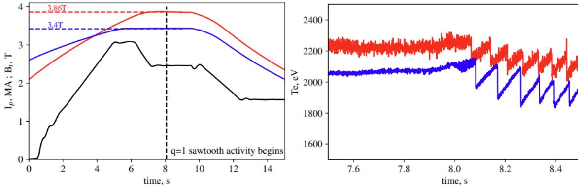
Figure 5: The effect of toroidal field ramp up on the target q -profile in cases of 3.4 T and 3.86 T. a) B_t (red: #97587, blue #97586) and I_p (black, the same for both discharges) waveforms, b) core electron temperature measured with the radiometer ECE, indicating the almost identical (within 20ms) start time of sawtooth activity.
