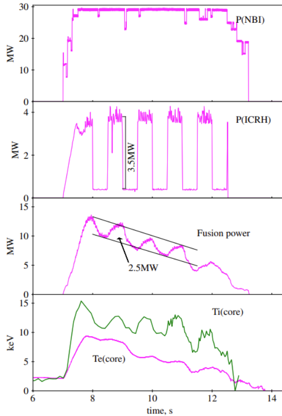
Figure 16: ICRF power modulation in tritium-rich pulse #99965 and the effect on the produced fusion power. From top to bottom: NBI power, ICRH power, fusion power output, core Te (ECE) and Ti (x-ray spectrometer) values – notable Ti modulation.
