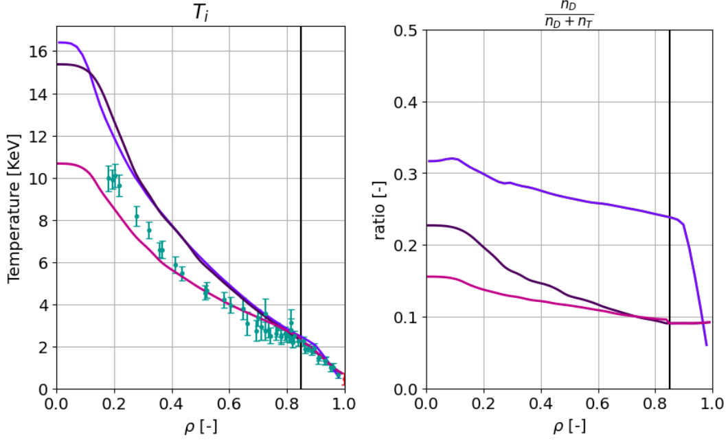
Figure 20: Kinetic profiles as measured, extrapolated and predicted imposing the experimental boundaries and heating as for the T-rich pulse #99971. The extrapolation performed before the experiment is shown in purple. The simulations performed after the experiment with and without the ad-hoc proxy for the electromagnetic stabilization effects are shown in pink and black respectively. The experimental data are shown in light green. The boundary condition is set at \rho_{\text{tor}}=0.85 , as marked by the vertical black line.
