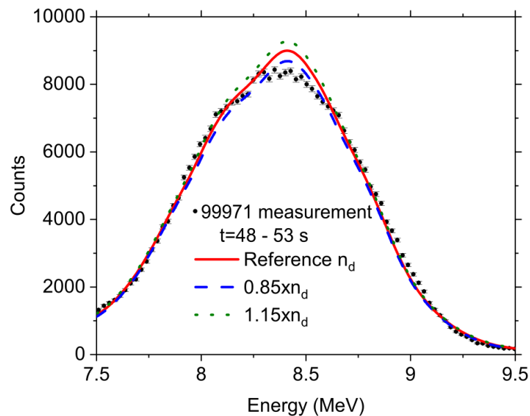
Figure 19: Neutron spectrum (shifted by 5.702 MeV from the ^{12}\text{C}(n,\alpha)^9\text{Be} reaction[33]) measured by the vertical line of sight diamond detector versus reconstructed spectra for different D/T plasma compositions. Reference n_D/n_e=15\%
