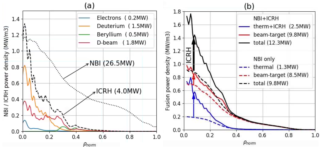
Figure 18: (a) NBI deposition (26.5MW) and ICRH power absorption profiles per species (4MW) computed with the ETS heating and current-drive workflow using the experimental parameters of the high-performance T-rich discharge #99971 at t=9\text{s} ; (b) Calculated fusion power profiles accounting for the heated distribution functions of all the plasma species with NBI+ICRH heating. The dashed curves represent the values obtained with NBI only heating.
