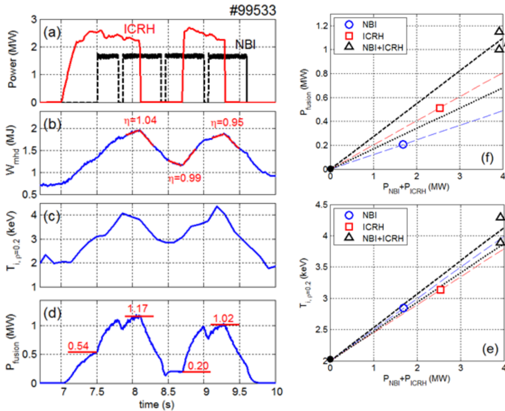
Figure 7: Time traces of main parameters in a T-rich L-mode discharge #99533 used to prove the n=1 D RF heating scheme: (a) ICRF and NBI power; (b) Plasma stored energy, with red highlighted line indicating where the break-in-slope analysis was performed; (c) Core ion temperature ( \rho=0.2 , crystal spectrometer); (d) Total fusion power. The right column shows the average core ion temperature (e) and the average fusion power (f) obtained with NBI-only ( t=8.6 s), ICRF-only ( t=7.5 s) and combined NBI+ICRF heating ( t=8.1 s and 9.3 s).
