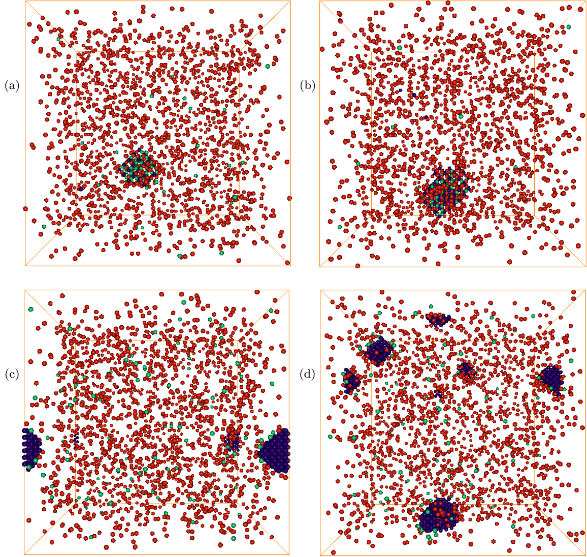
FIG. 10: MC simulations for \text{WRe}_{1.5}\text{Os}_{0.1} with different vacancy concentrations: a) 0.05%, b) 0.1%, c) 0.2% and d) 0.5%
