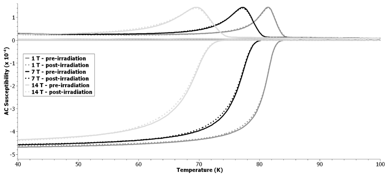
S 6. AC susceptibility versus temperature for multi-filamentary repeat sample 2 prior to and post 1 MGy gamma irradiation - susceptibility values at 1, 7 and 14 T
