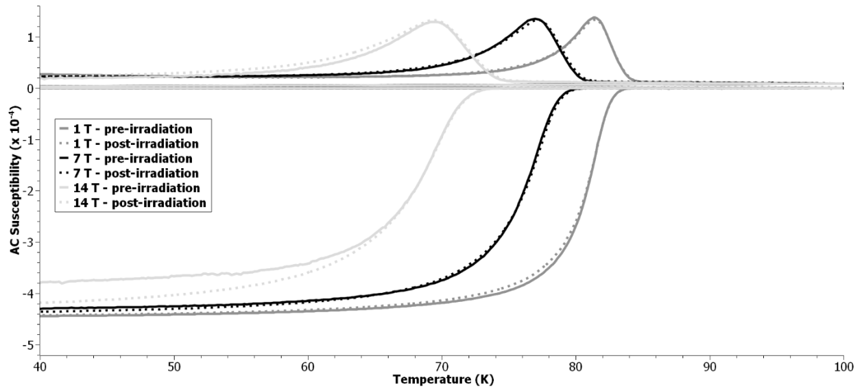
S 5. AC susceptibility versus temperature for multi-filamentary repeat sample 1 prior to and post 1 MGy gamma irradiation - susceptibility values at 1, 7 and 14 T
