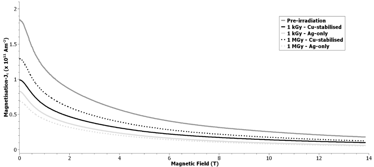
Fig. 13 Magnetisation critical current density versus magnetic field for the GdYBCO 15 % Zr tape prior to gamma irradiation, and the Cu-stabilised and Ag-only samples after 1 kGy and 1 MGy gamma irradiation – J_c values calculated at 20 K [10]
