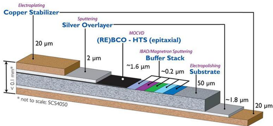
Fig. 1 Schematic diagram of a SuperPower SCS4050 REBCO coated conductor tape [21]
