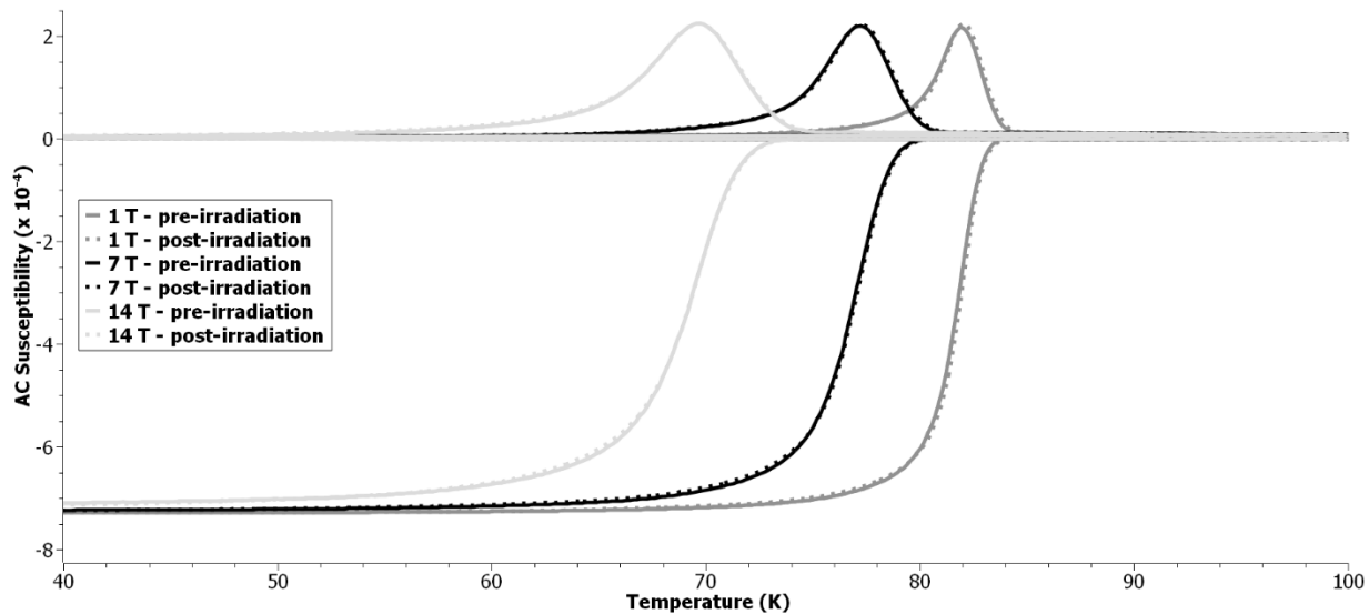
S 4. AC susceptibility versus temperature for mono-filamentary repeat sample 2 prior to and post 5 MGy gamma irradiation - susceptibility values at 1, 7 and 14 T
