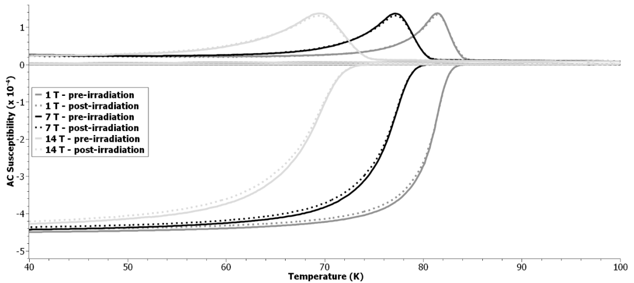
S 8. AC susceptibility versus temperature for multi-filamentary repeat sample 3 prior to and post 5 MGy gamma irradiation - susceptibility values at 1, 7 and 14 T
