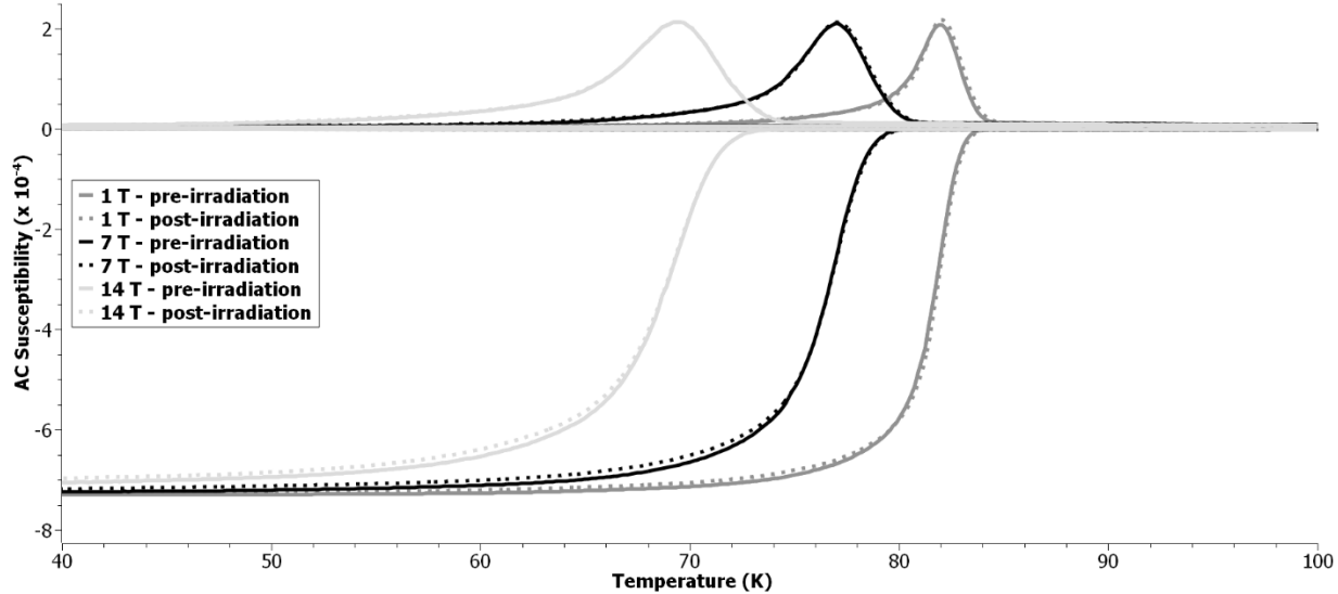
S 3. AC susceptibility versus temperature for mono-filamentary repeat sample 1 prior to and post 5 MGy gamma irradiation - susceptibility values at 1, 7 and 14 T
