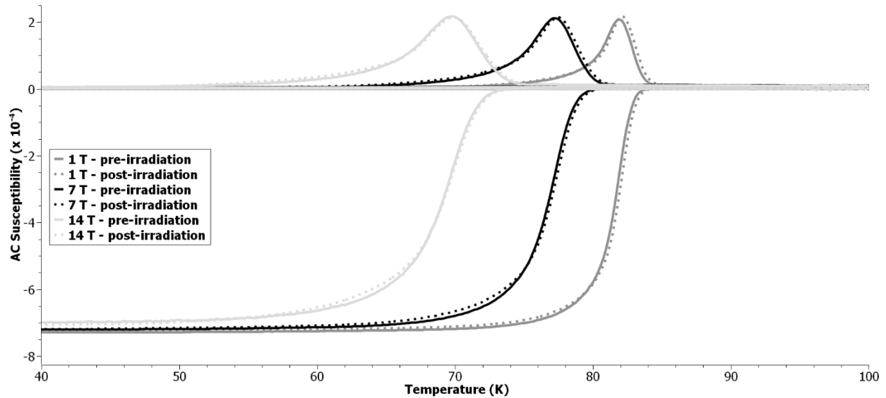
S 2. AC susceptibility versus temperature for mono-filamentary repeat sample 2 prior to and post 1 MGy gamma irradiation - susceptibility values at 1, 7 and 14 T
