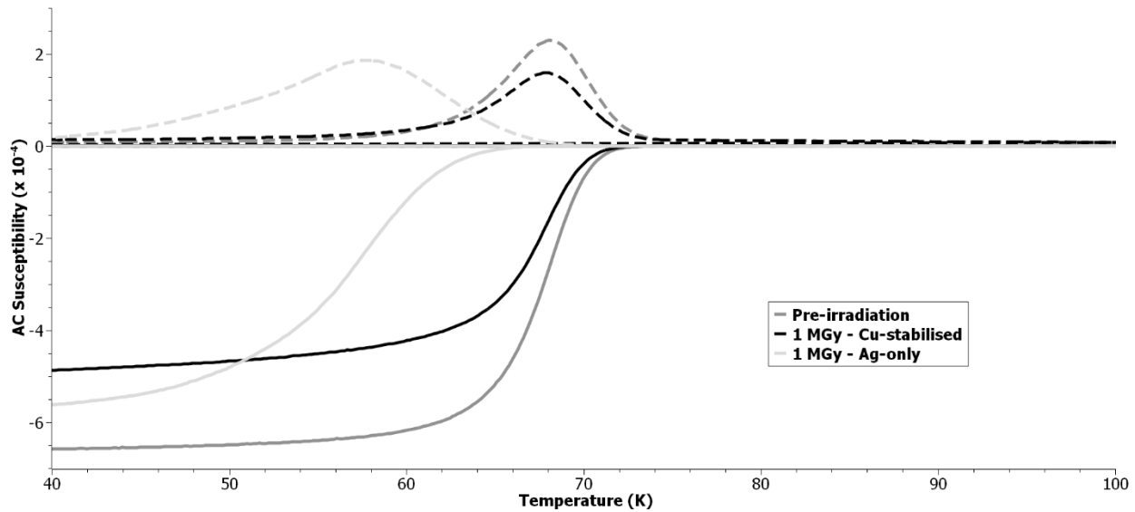
Fig. 15 AC susceptibility versus temperature for the GdYBCO 15 % Zr tape prior to gamma irradiation, and the Cu-stabilised and Ag-only samples after 1 MGy gamma irradiation – susceptibility values at 14 T [10]
