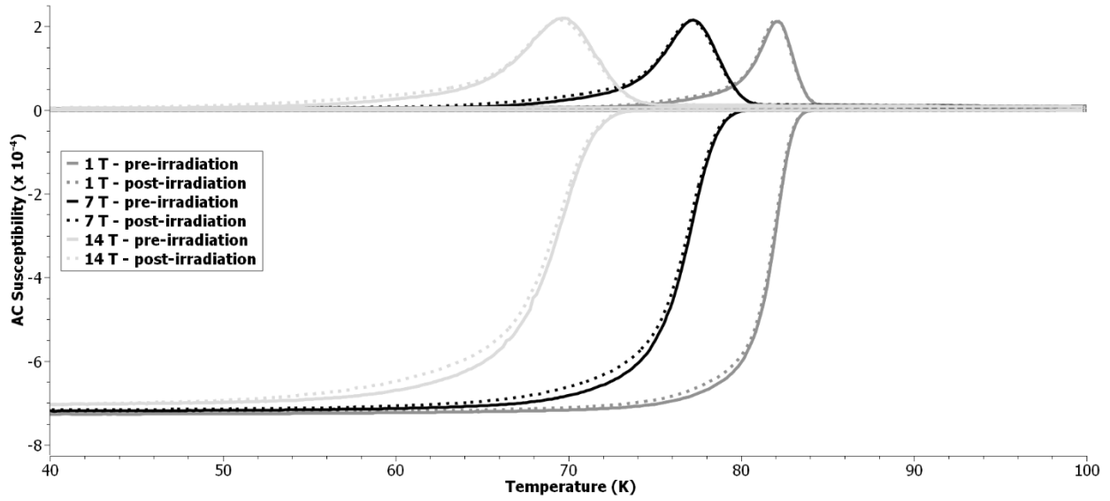
S 1. AC susceptibility versus temperature for mono-filamentary repeat sample 1 prior to and post 1 MGy gamma irradiation - susceptibility values at 1, 7 and 14 T
