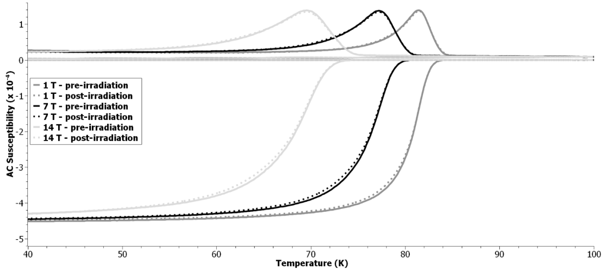
S 7. AC susceptibility versus temperature for multi-filamentary repeat sample 1 prior to and post 5 MGy gamma irradiation - susceptibility values at 1, 7 and 14 T
