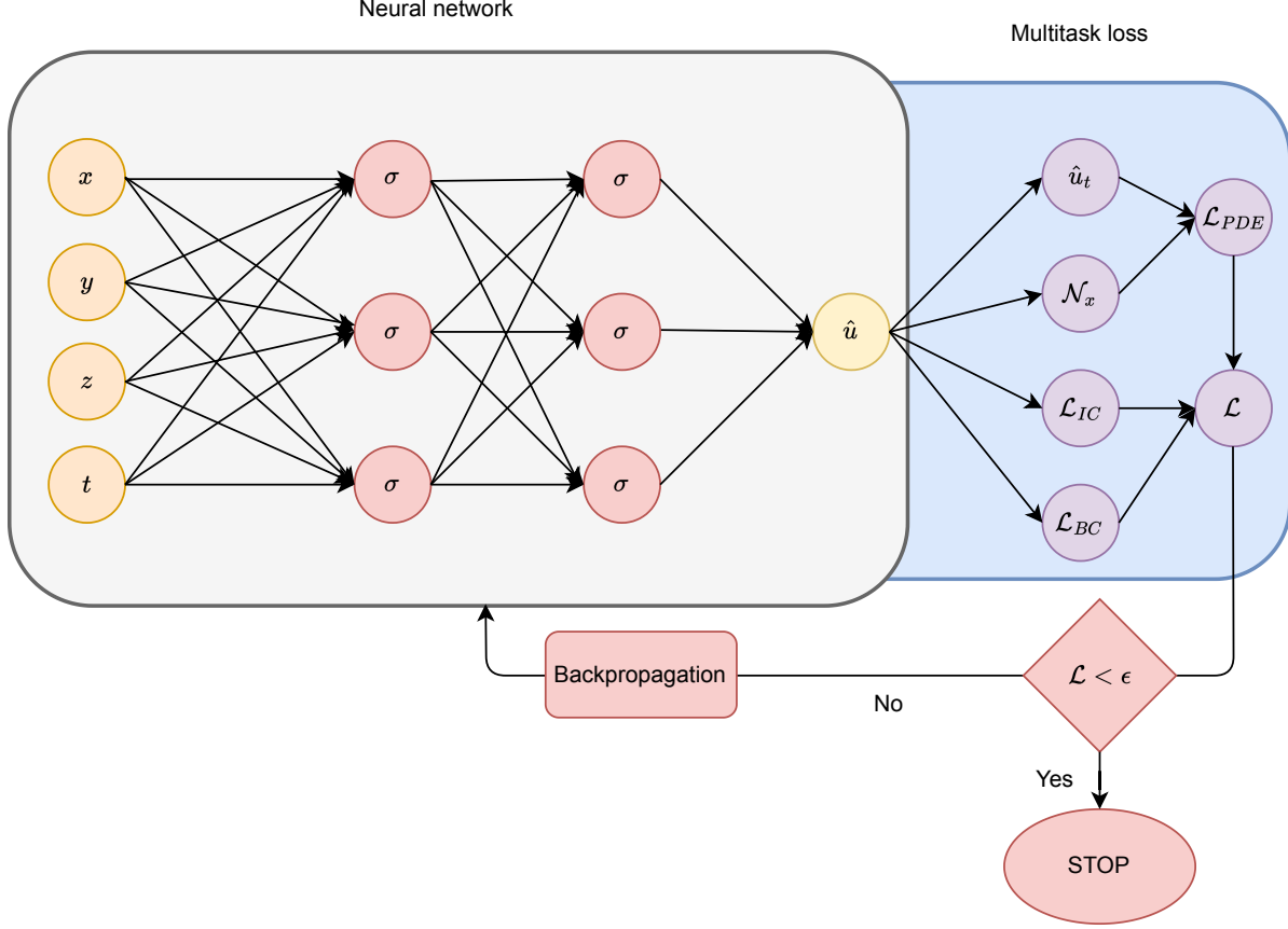
Figure 2: The architecture of a PINN with two hidden layers for a 3D spatio-temporal forward problem. Here the inputs are x, y, z and t , \sigma is the activated neuron and \hat{u} is the predicted output or the solution to the PDE.
