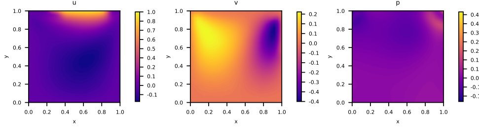
Figure 13: Baseline PINN predicted solution of the lid-driven cavity.
