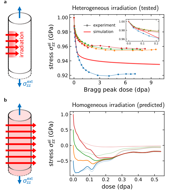
Fig. 4: Stress relaxation under heterogeneous and homogeneous irradiation. a , Comparison of four irradiation-induced stress relaxation experiments to the parameter-free simulation using the virtual wire model under an initial uniaxial tensile stress of 1 GPa. The model predicts a small degree of relaxation, in agreement with experiment, due to the small volume fraction of the irradiated volume. b , Predicted stress relaxation curves for a hypothetical homogeneous irradiation scenario under various initial uniaxial tensile and compressive stresses. Most of the relaxation is predicted to occur within the first 0.3 dpa.
