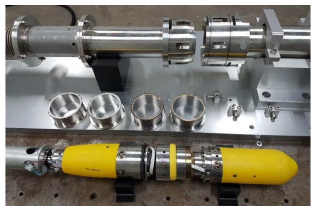
Fig. 4 PoP cutting tool and cut 316L and P91 samples
