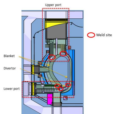
Fig. 1 First Wall Service Joining scenario
