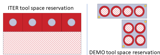
Fig. 8 ITER NB cutting and welding tool vs DEMO in-bore tool operating space
