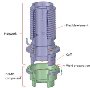
Fig. 3 Laser Bore Joint
