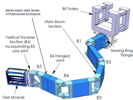
Figure 2: Octant 1 Boom Joints
