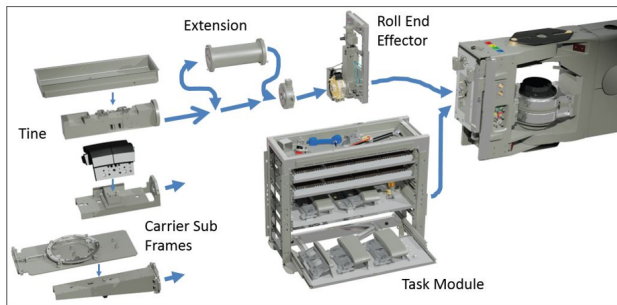
Figure 3: Octant 1 Boom End Effectors
