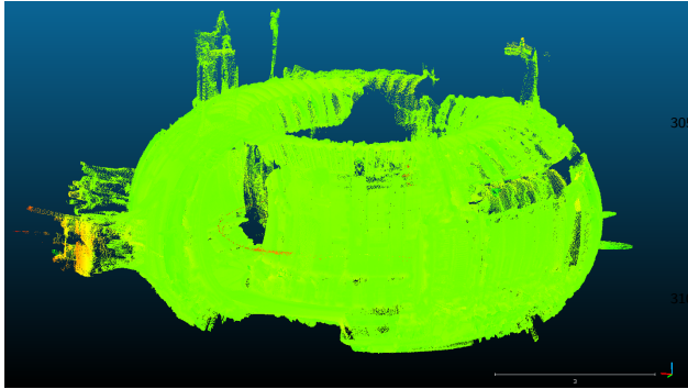
Figure 7: Heatmap of Pointcloud-CAD distances, showing outliers with over 15mm difference in orange and red. The red streak through the middle of the Torus comes from the LIDAR accidentally picking up the edge of the Boom during measurement.
