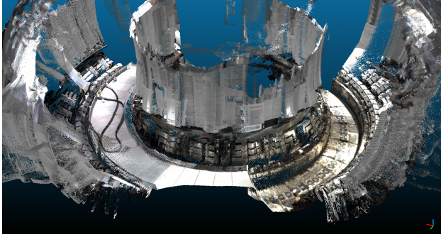
Figure 5: Section of coloured pointcloud of JET vessel inner wall, reconstructed using Boom kinematics.
