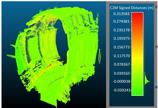
Figure 1: Heatmap and histogram of Cloud-to-Mesh distances between NABU dataset and JET CAD model [3]
