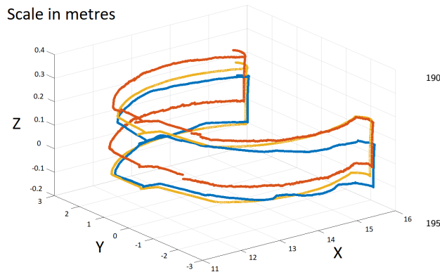
Figure 4: VO path in Blue, ORB path in Orange, Boom path in Yellow. All three data sources have the same starting position in Z. Note scale on Z-axis.
