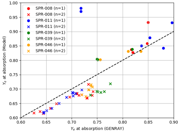
Figure 7. Predicted Y value at absorption (y axis) vs value from GENRAY for rays giving optimal current drive. The dashed black line shows where they are equal. There is reasonable agreement with a mean absolute error of 0.03.
