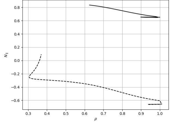
Figure 8. N_{\parallel} evolution across the ray trajectory for two rays giving maximum current drive at \rho = 0.45 (dashed) and \rho = 0.75 (solid) for SPR-008. Both rays start with |N_{\parallel}| \sim 0.65 . The ray traces continue beyond the point of absorption but there is no power left in the ray.
