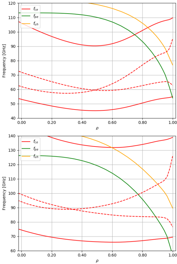
Figure 9. Model of EBW absorption on midplane for SPR-008 (top) and SPR-046 (bottom) for N_{\parallel} = 0.65 . The cold cyclotron harmonic frequencies (red) and predicted upshift from 1 st harmonic/ downshift from 2 nd harmonic from (3) (dashed red) are shown. The plasma frequency (green) and upper hybrid frequency (orange) are also shown.
