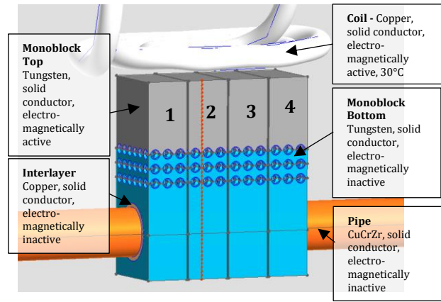
Fig. 13 – Screenshot of the monoblock geometry in Flux. The different volume regions and their corresponding settings are labelled. The dashed-red line along the face of monoblock 2 is used to produce the temperature plot in Figure 15.
