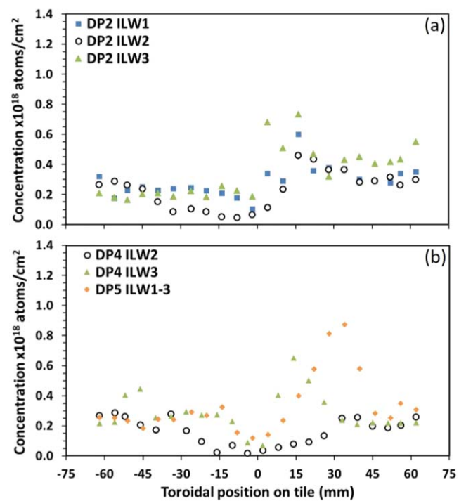
Figure 4. Deuterium areal concentration on dump plate (DP) tiles. (a) DP2 after ILW1, ILW2 and ILW3, (b) DP4 after ILW2, ILW3 and DP5 after ILW1-3. 0 mm is the centre of the tile. Positive values are to the right of the tile and negative values to the left of the tile, when following a poloidal line from the inner wall up to the dump plates.
