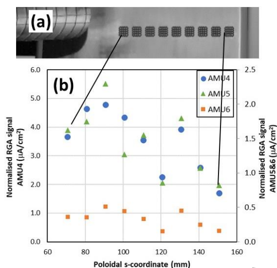
Figure 11: (a) Schematic showing poloidal position of 4x4 LID-QMS measurements. The location of the measurements are shown in Figure 2(b-iv). (b) Normalised AMU4 ( D_2 ), AMU5 (DT) and AMU6 ( T_2 ) QMS signal indicating qualitative fuel retention distribution in poloidal direction. S-coordinate is the distance along the surface of the tile starting at 0 mm on top left corner of HFGC tile, see Figure 2(a).
